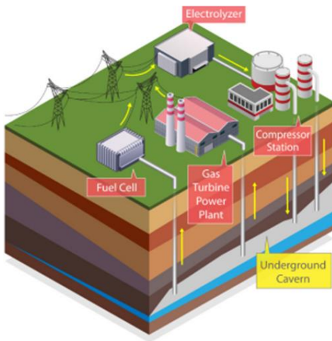
Figure 18: Hydrogen energy storage systems involve the use of electrolyzers to produce hydrogen from excess power on the grid, bulk storage, followed by power generation using fuel cells or turbines.
