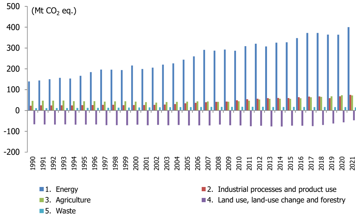
Figure 2.9 GHG emission trend by sectors, 1990-2021
