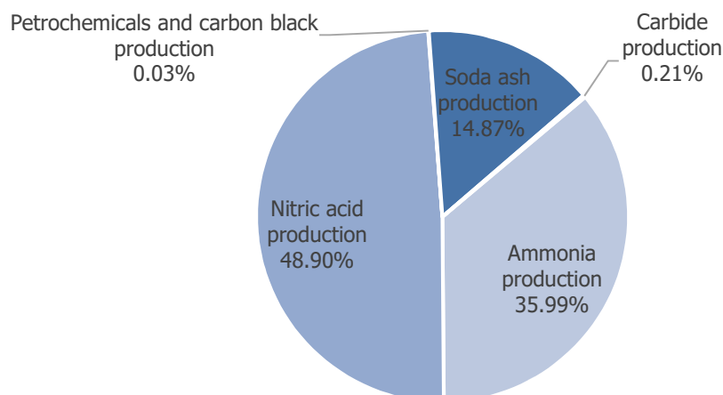
Figure 4.11 CO 2 emissions from chemical industry, 2021
