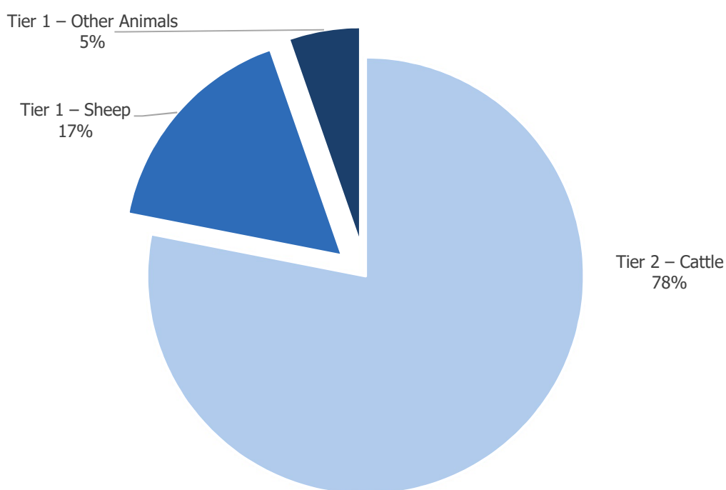
Figure 5.6 Enteric Fermentation Emission Sources, 2021
