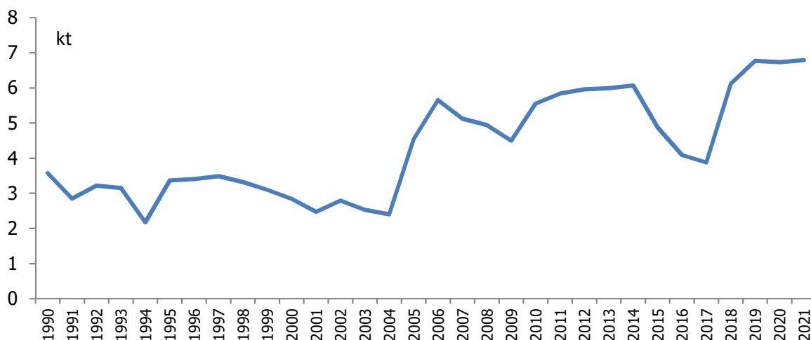
Figure 4.13 N_2O emissions from nitric acid productions, 1990-2021
