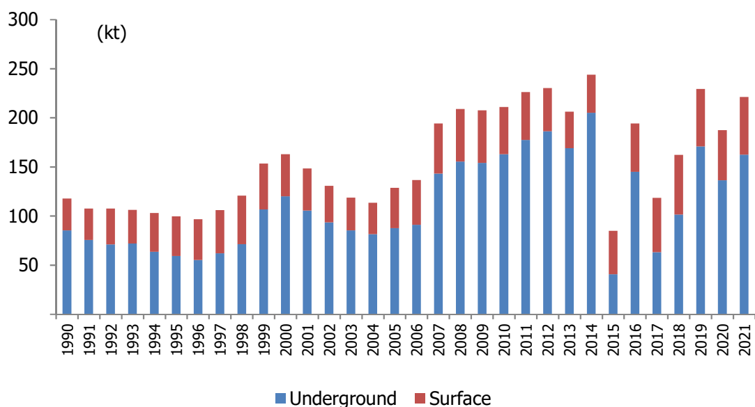
Figure 3.33 CH 4 emissions from coal mining, 1990-2021
