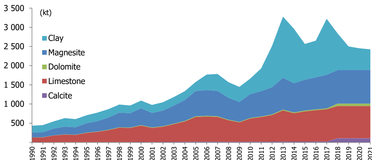
Figure 4.8 CO 2 emissions, by raw materials type, from ceramics, 1990-2021
