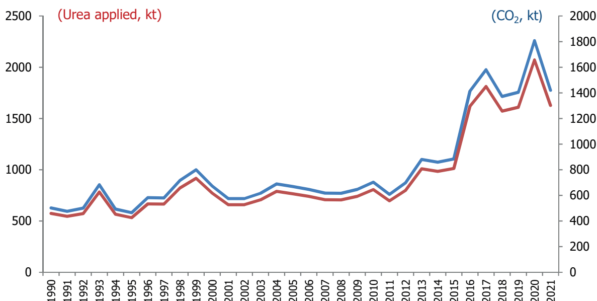
Figure 5.12 Urea application and emitted CO 2 , 1990–2021
