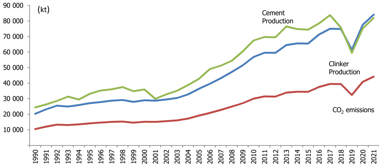
Figure 4.4 Trend at clinker, cement production and related CO 2 emissions, 1990-2021
