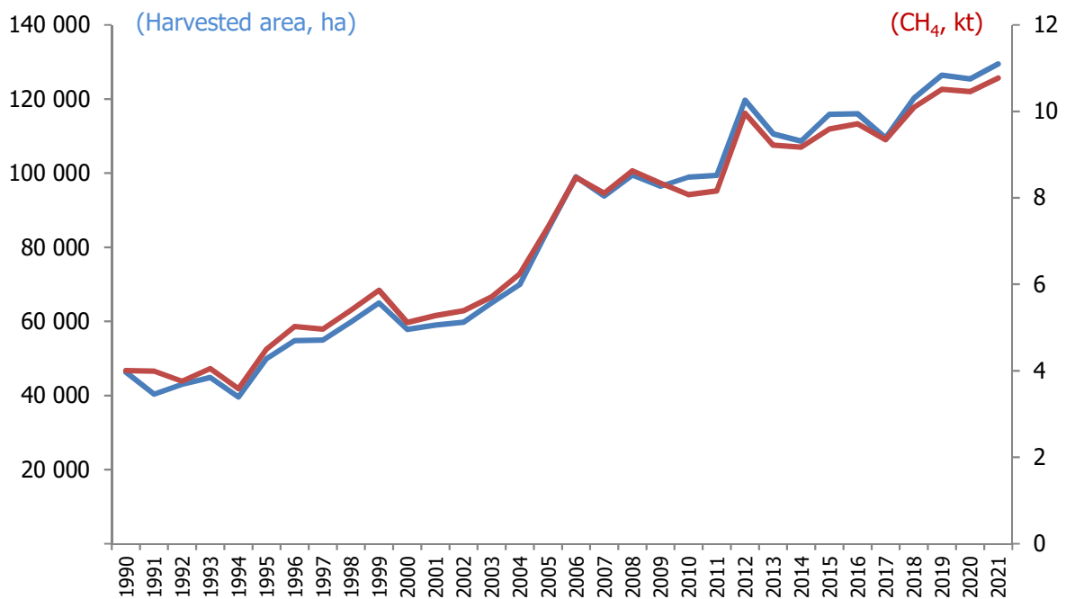
Figure 5.9 Harvested area and emitted CH 4 for rice cultivation, 1990–2021
