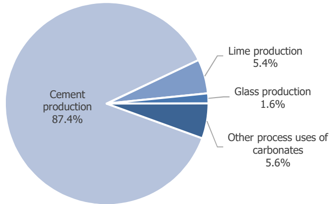
Figure 4.3 Share of CO 2 emissions from mineral production, 2021
