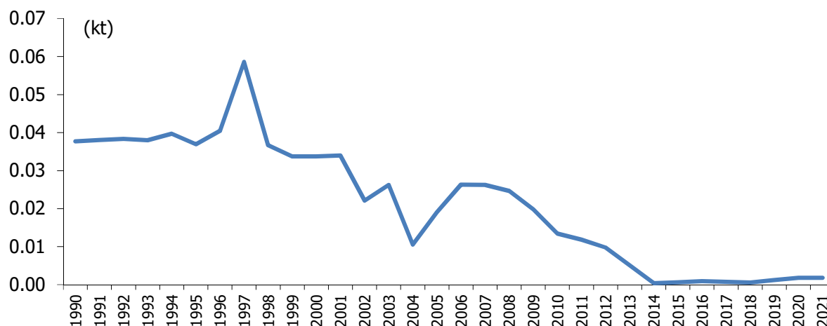
Figure 7.8 N 2 O emissions from open burning of waste, 1990-2021
