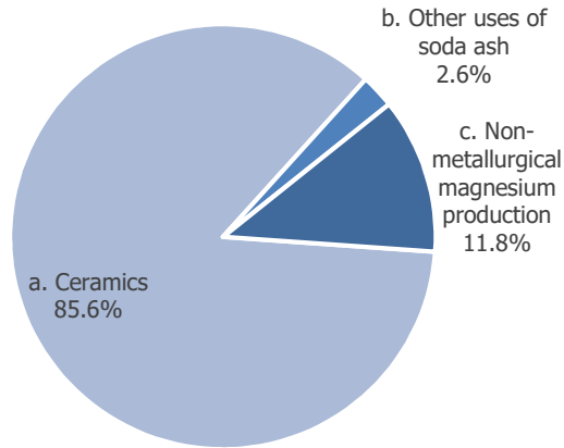
Figure 4.7 CO 2 emissions from other uses of carbonates, 1990-2021
