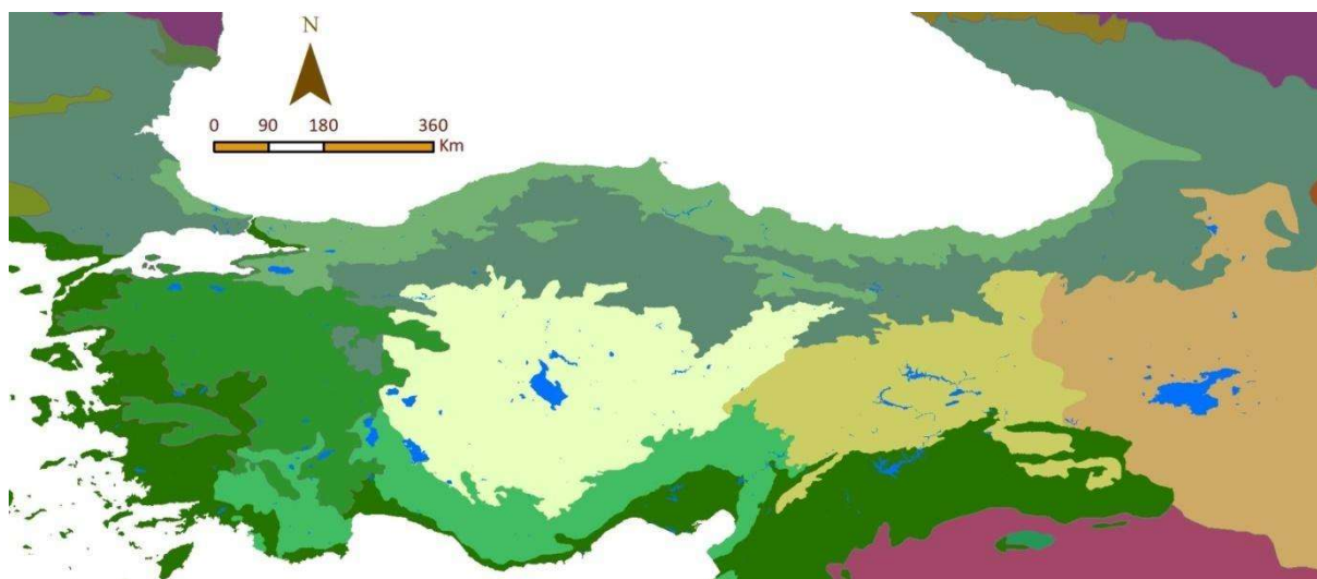
Figure 6.2 The ecoregions in Türkiye (Serengil, 2018)
