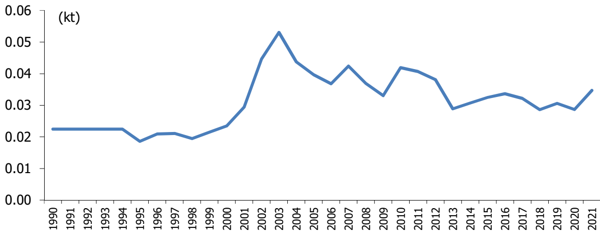
Figure 7.5 N 2 O emissions from composting, 1990-2021
