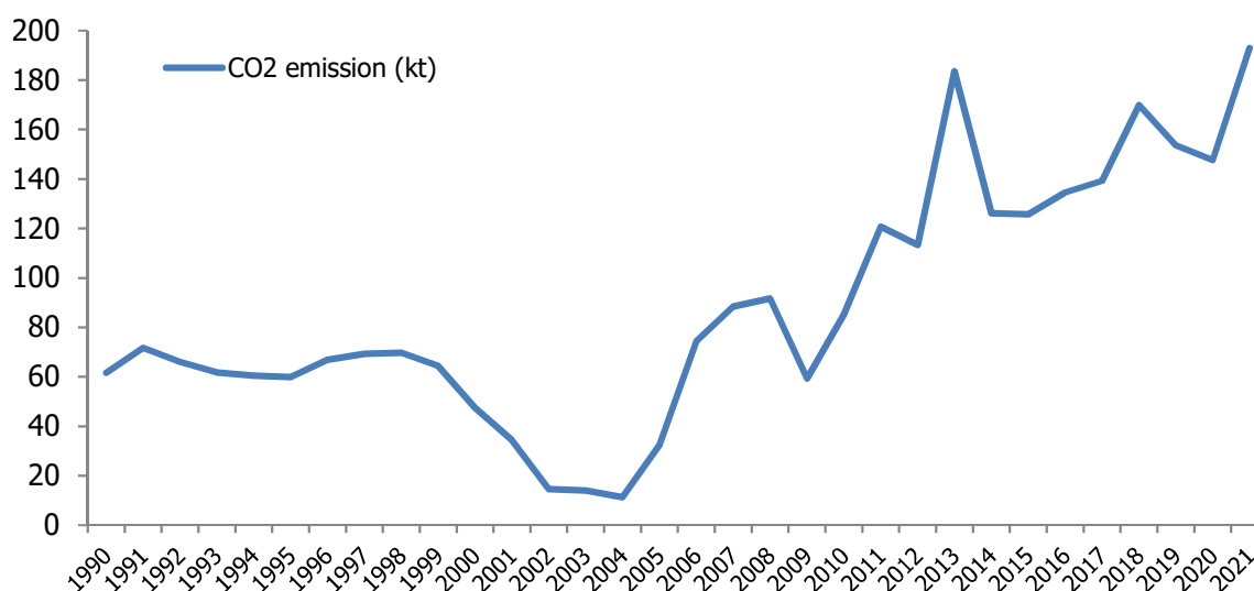
Figure 4.20 CO 2 emissions from ferroalloys production, 1990-2021
