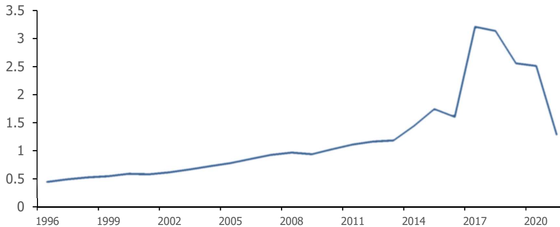
Figure 4.25 SF 6 emissions, 1996-2021
