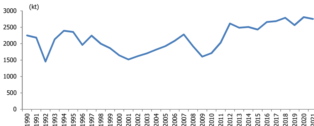
Figure 4.5 CO 2 emissions from lime production, 1990-2021
