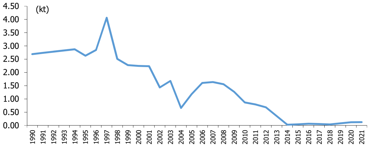
Figure 7.7 CH 4 emissions from open burning of waste, 1990-2021
