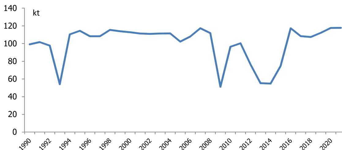
Figure 4.21 CO 2 emissions from aluminium production, 1990-2021
