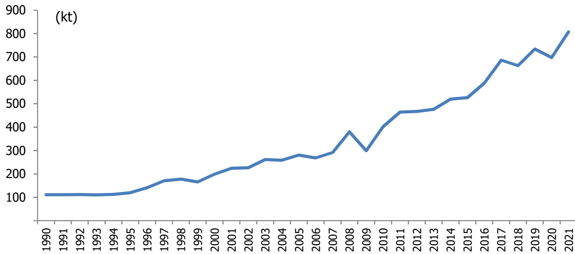
Figure 4.6 CO 2 emissions from glass production, 1990-2021
