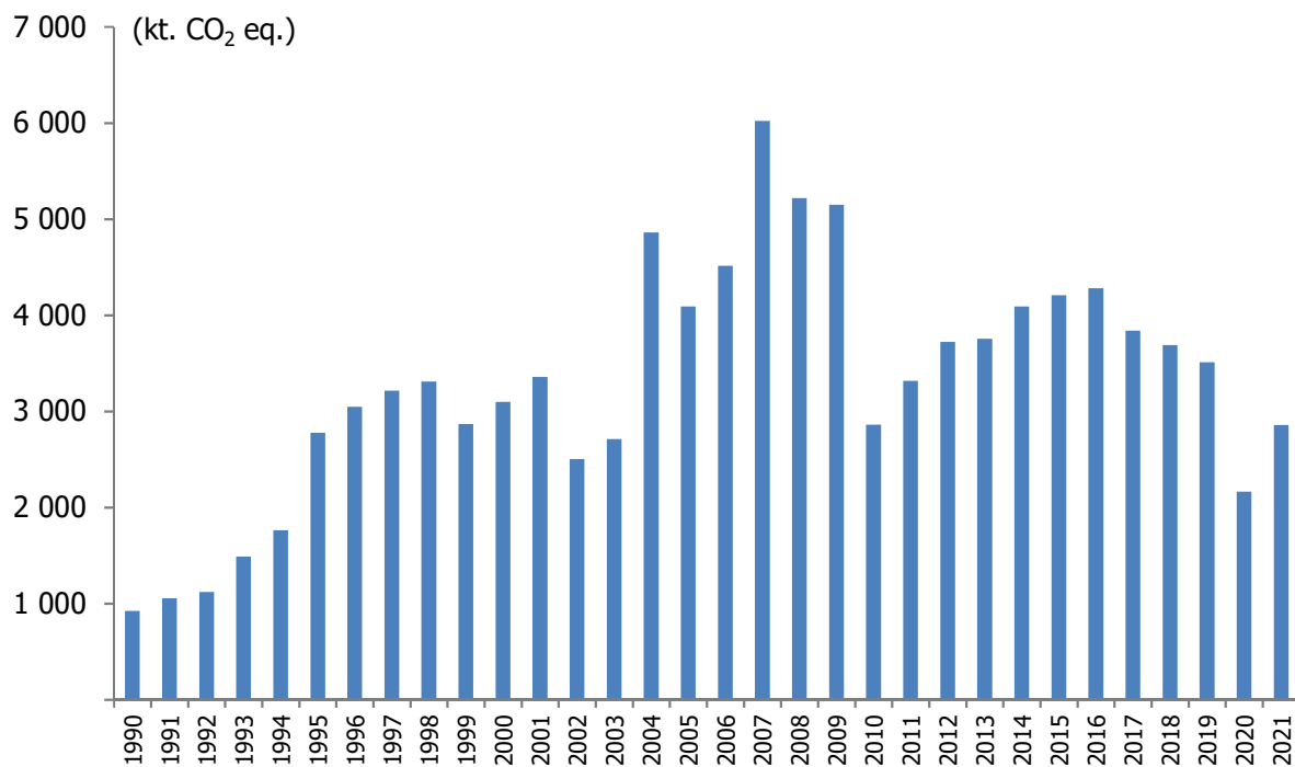
Figure 3.19 GHG emissions for domestic aviation, 1990-2021
