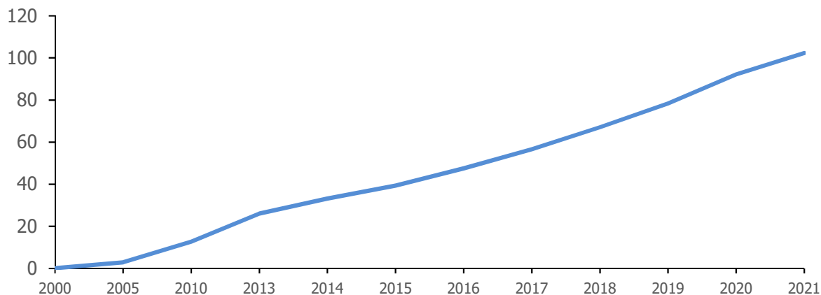
Figure 4.24 HFC-227ea Emissions (tonnes), 2000-2021
