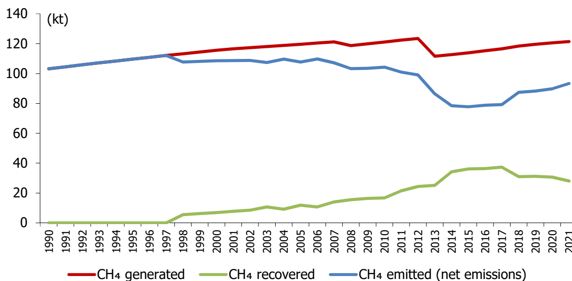
Figure 7.10 CH 4 emissions from domestic wastewater, 1990-2021
