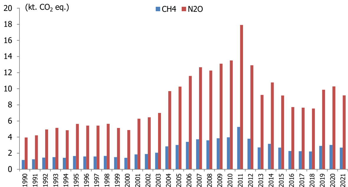
Figure 3.30 CH 4 and N 2 O emissions from domestic water-borne navigation, 1990-2021
