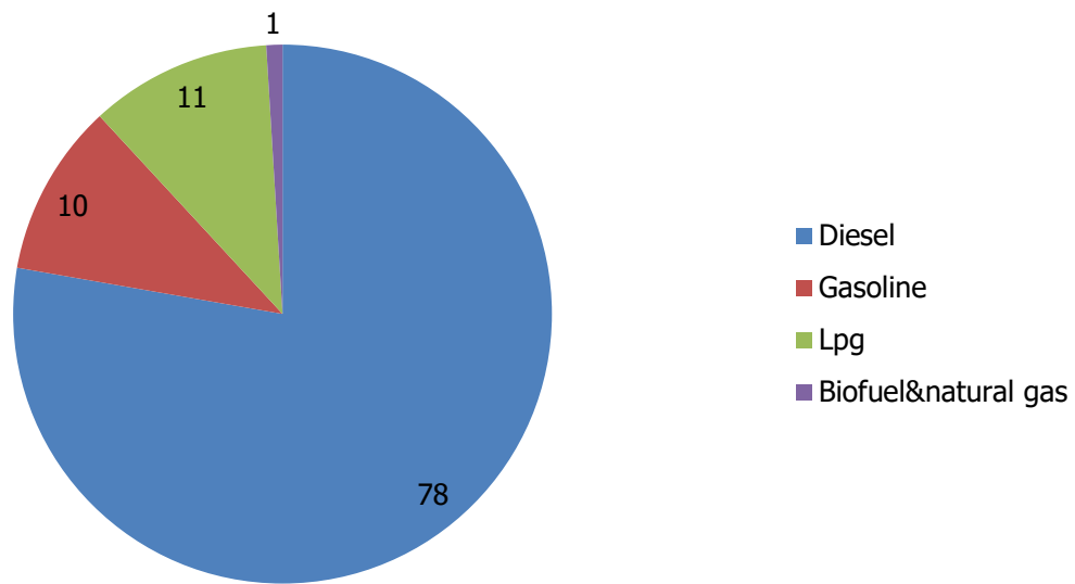
Figure 3.26 CO 2 emission distributions by fuel types (%), 2021
