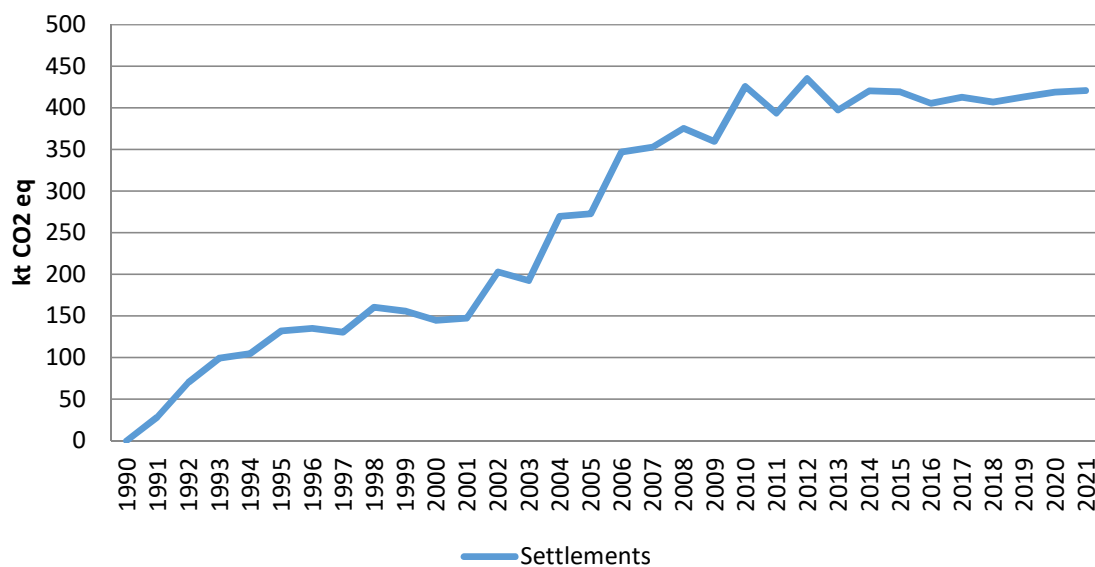
Figure 6.16 The change in net emissions in settlements
