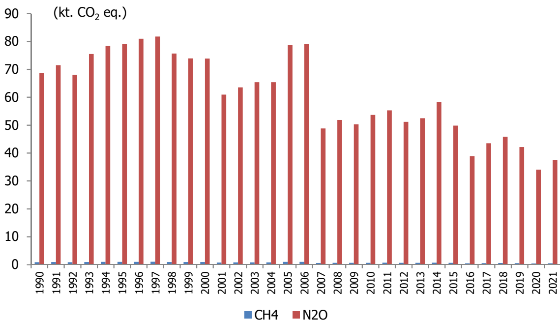
Figure 3.28 CH 4 and N 2 O emissions from railways, 1990-2021
