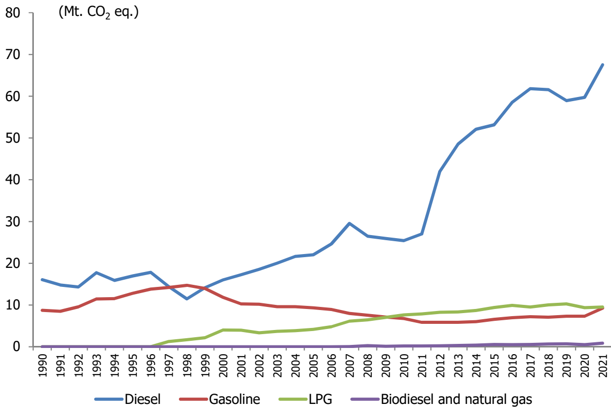
Figure 3.16 Emission distributions by fuel types in road transportation, 1990-2021
