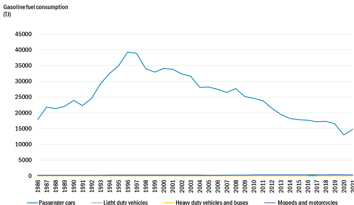
Figure 3.2.17: Gasoline fuel consumption per vehicle type for road transport 1986–2021.
