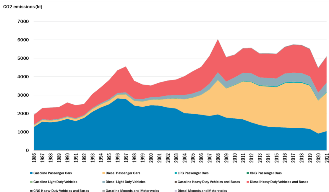
Figure 3.2.9: CO 2 emissions (kt) per vehicle type for road transport 1986–2021.
