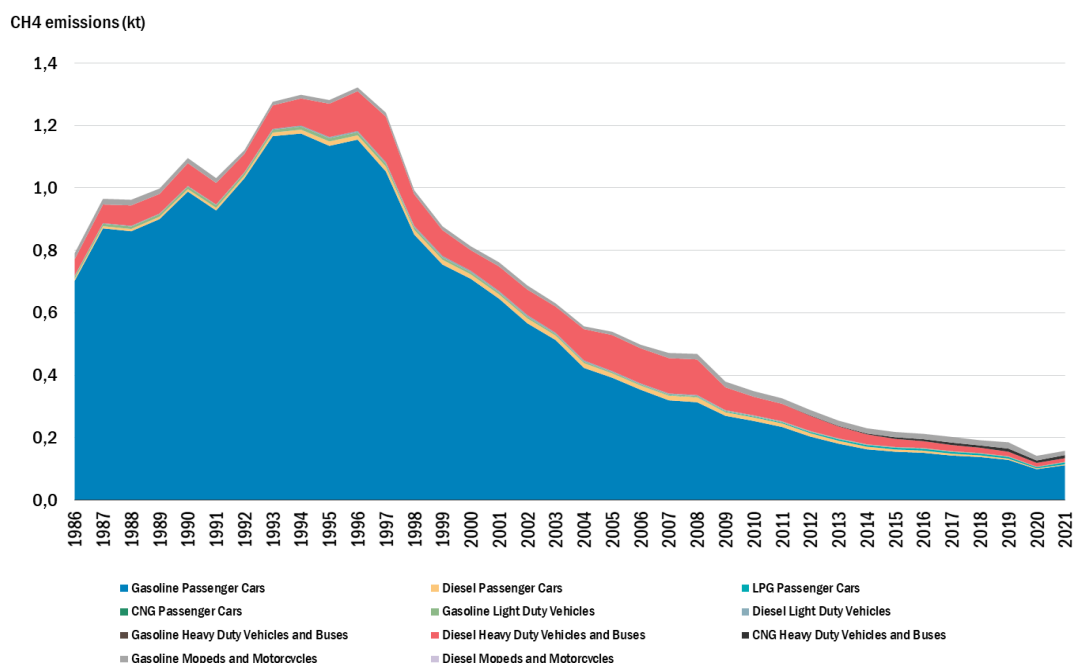
Figure 3.2.13: CH 4 emissions (kt) per vehicle type for road transport 1986–2021.
