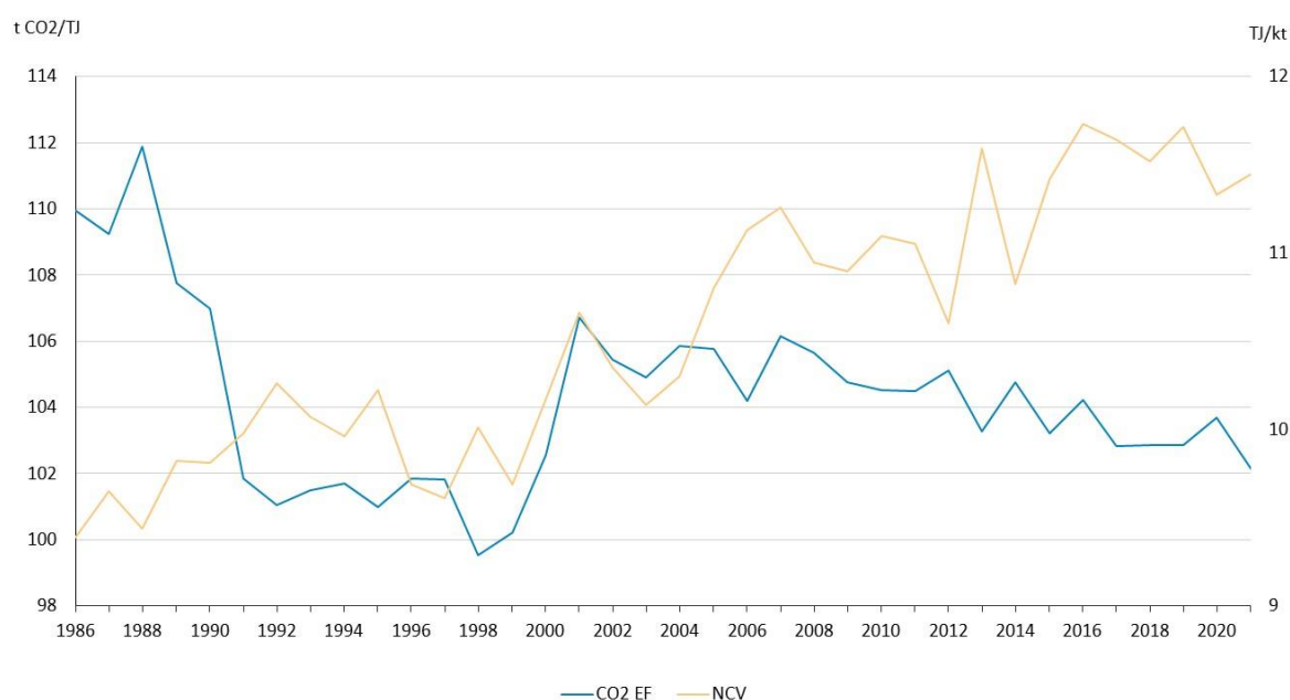
Figure 3.2.1: CO 2 EF and NCV for domestic lignite from Velenje pit for 1986-2021.
