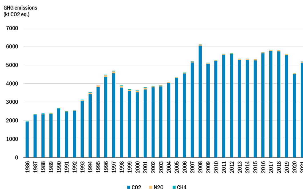
Figure 3.2.8: CO 2 , N 2 O and CH 4 emissions for road transport 1986–2021.
