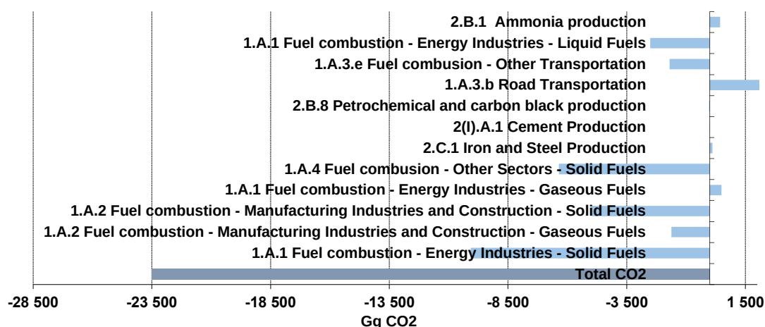
Figure 2.7: Absolute change of CO 2 emissions by large key categories 1990 to 2021
