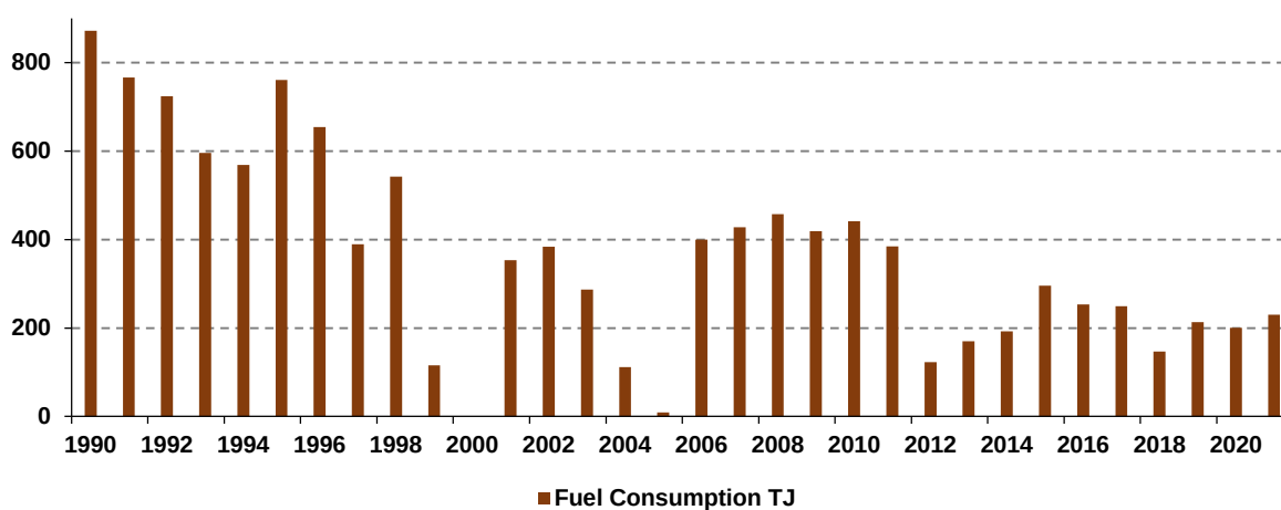
Figure 3.17: Overview of diesel / oil consumption (TJ) for shipping transport in 1990 – 2021
