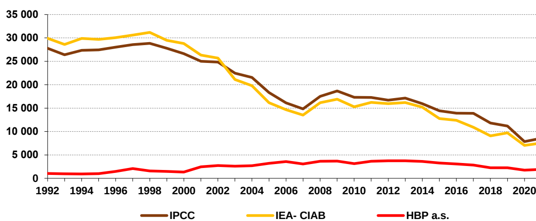
Figure 3.15: Comparison of CH 4 (t) emissions trends in the Slovak Republic in years 1992 – 2021
