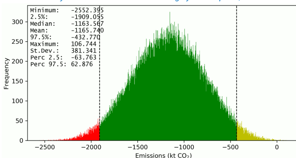
Figure A6.2.2: Probability distribution function for the category 4.B Cropland, 2021
