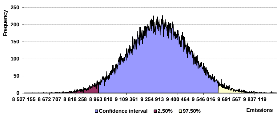
Figure 4.11: Probability density function for 2.A.4.d (t of \text{CO}_2 eq.)
