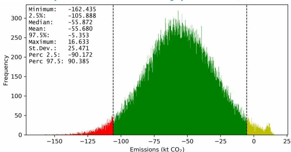
Figure A6.2.3: Probability distribution function for the category 4.C Grassland, 2021
