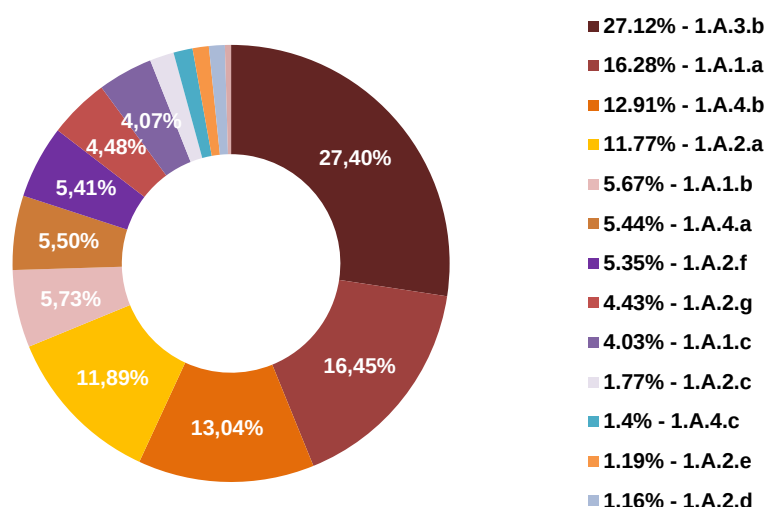
Figure 3.6: The share of emissions in CO 2 eq. on different subcategories within 1.A in 2021
