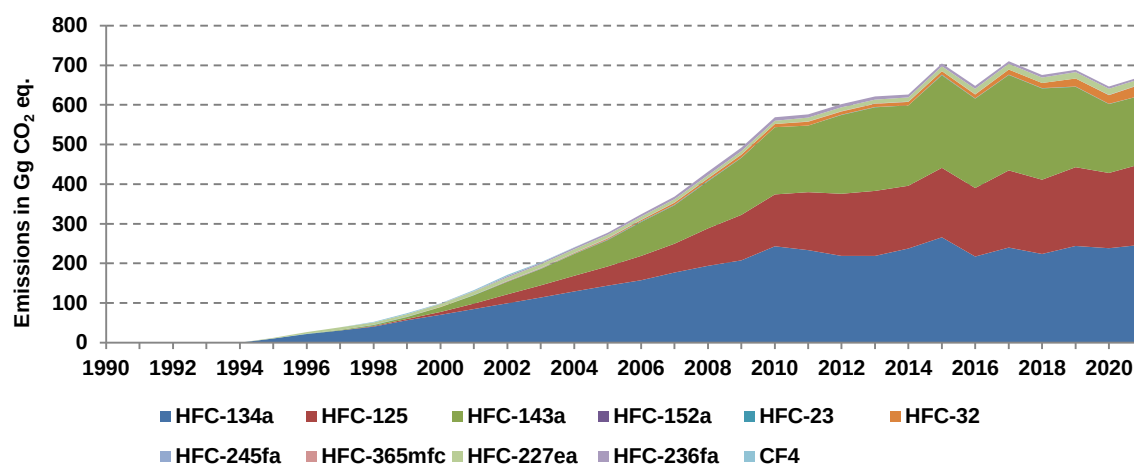
Figure 4.32: Trend in individual F-gases in 1990 – 2021
