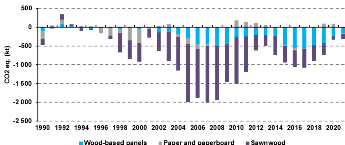
Figure 6.26: CO 2 emissions (positive values) and removals (negative values) from HWP in Slovakia in 1990 – 2021 originating from Forest Land
