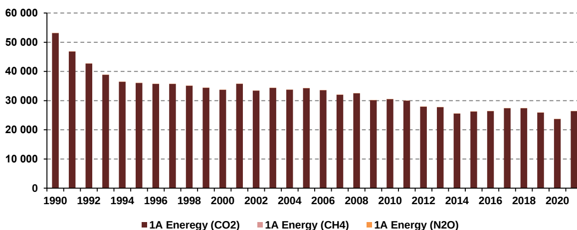
Figure 3.3: Trend in aggregated emissions by gases within the Energy sector in 1990 – 2021 (Gg of CO 2 eq.)
