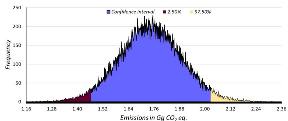
Figure 4.36: Probability density function for 2.F.2 (t of CO 2 eq.)
