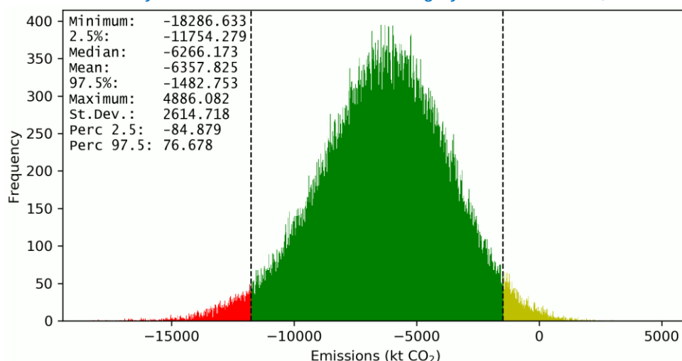
Figure A6.2.1: Probability distribution function for the category 4.A Forest Land, 2021
