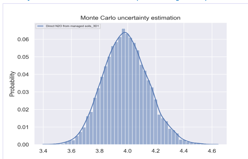
Figure 5.12: Probability distribution function for 3.D.1 (x-axis in Gg of N 2 O)
