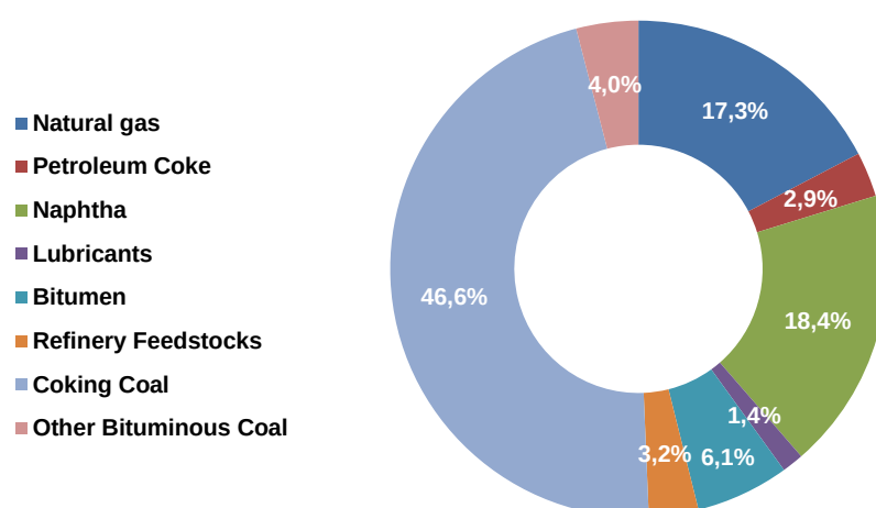
Figure 3.13: The share of carbon for feedstock and non-energy use in 2021
