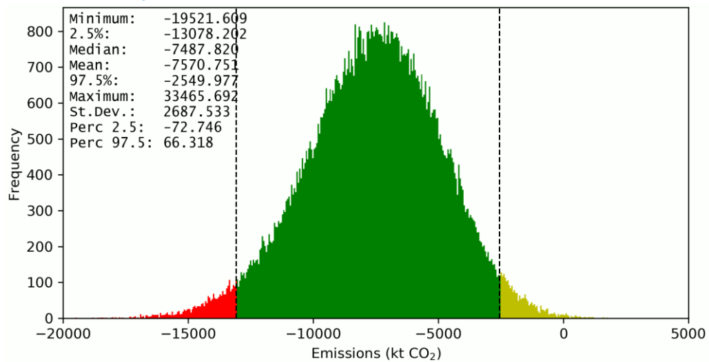
Figure A6.2.7: Probability distribution function for LULUCF sector, 2021
