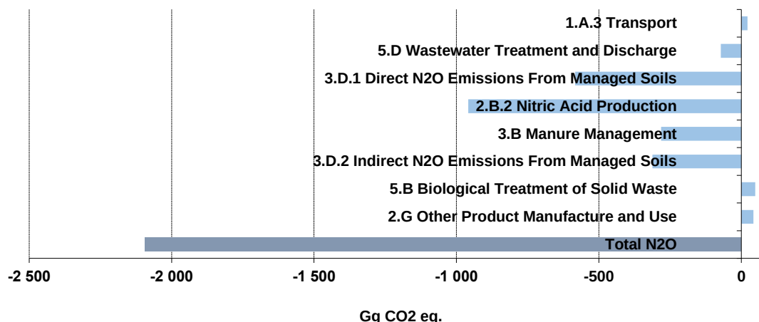
Figure 2.9: Absolute change of N 2 O emissions by large key categories 1990 to 2021
