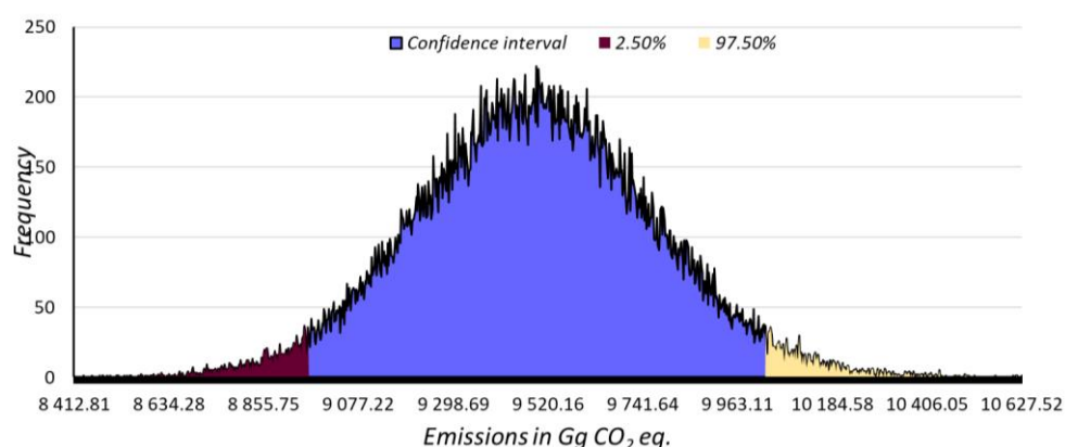
Figure 4.4: Probability density function for IPPU sector (t of CO 2 eq.)
