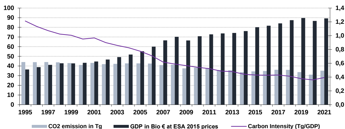
Figure 1.1: Comparison of CO 2 emissions per GDP (carbon intensity) in 1995 – 2021
