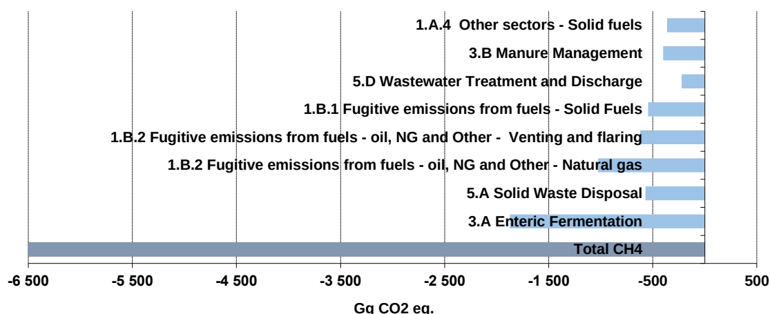
Figure 2.8: Absolute change of CH 4 emissions by large key categories 1990 to 2021
