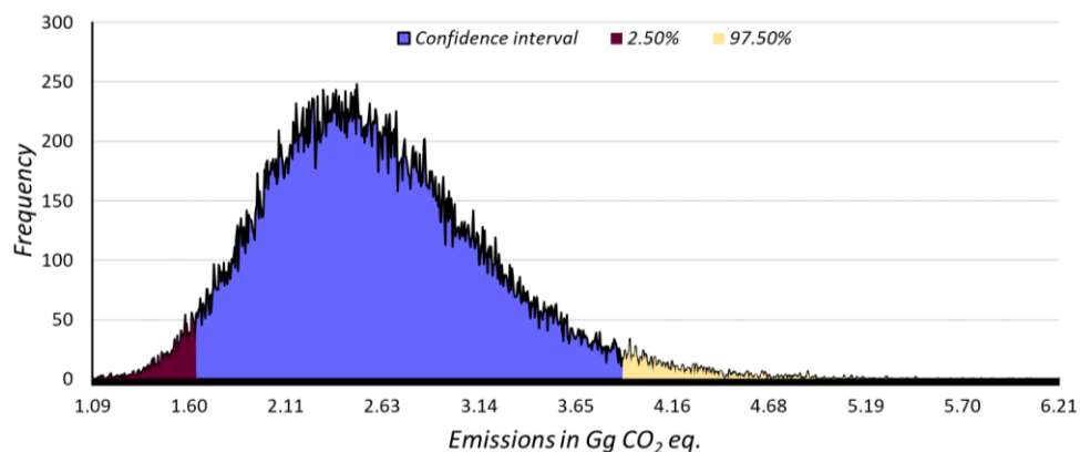
Figure 4.29: Probability density function for 2.D.2 (t of CO 2 eq.)
