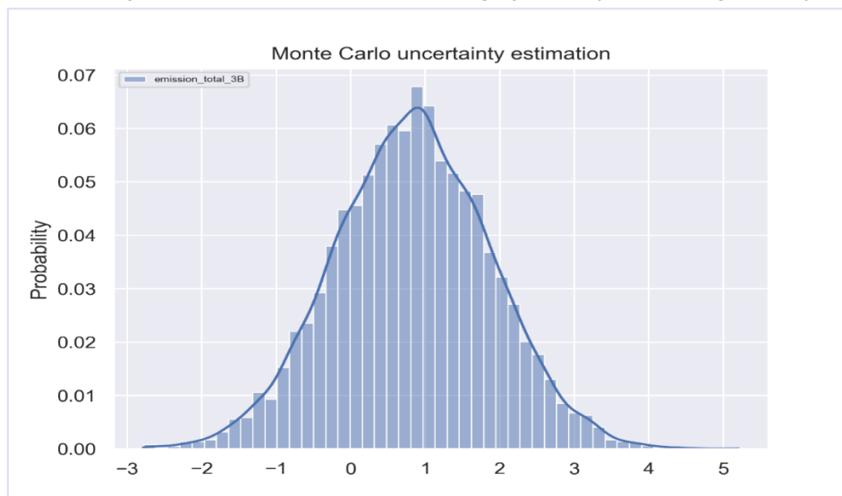
Figure 5.11: Probability distribution function for the category 3.B.2 (x-axis in Gg of N 2 O)
