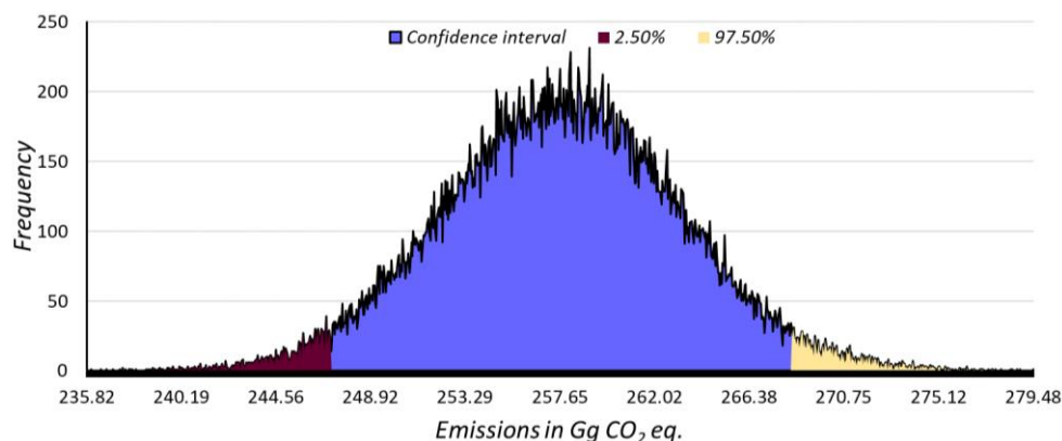
Figure 4.10: Probability density function for 2.A.4.c (t of CO 2 eq.)
