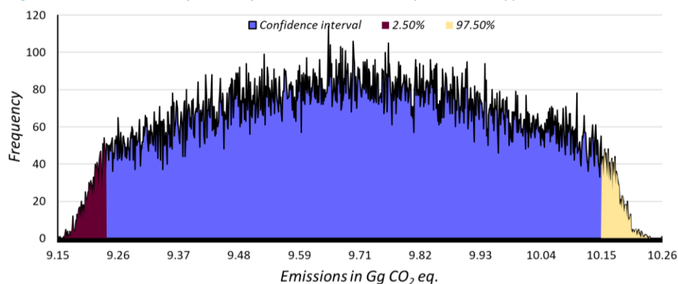
Figure 4.30: Probability density function for 2.D.3 (t of CO 2 eq.)
