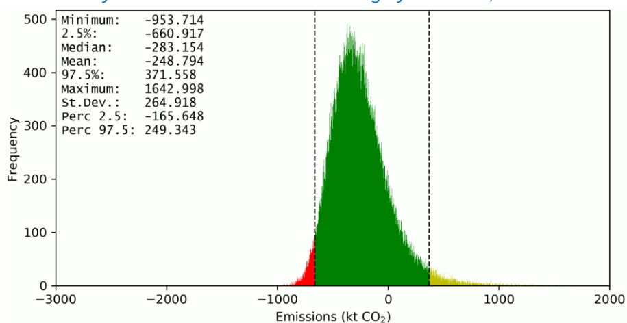
Figure A6.2.6: Probability distribution function for the category 4.G HWP, 2021
