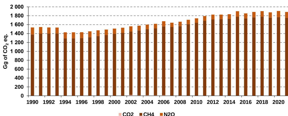
Figure 7.3: Trend in aggregated emissions by gases within the waste in 1990 – 2021
