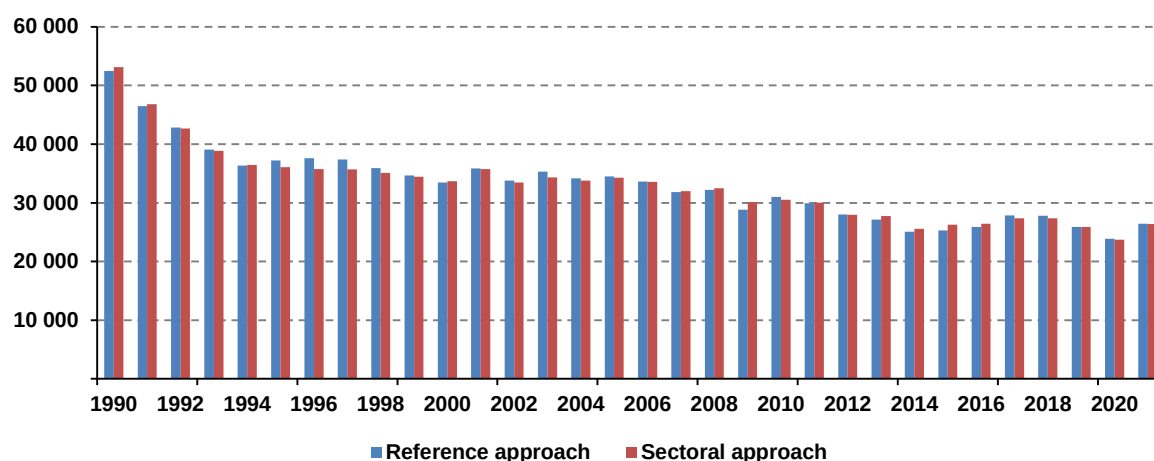
Figure 3.11: Difference between the reference and sectoral approaches CO 2 emissions (in Gg) in 1990 – 2021
