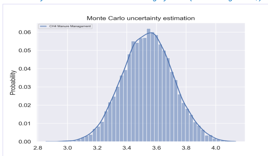
Figure 5.10: Probability distribution function for the category 3.B.1 (x-axis in Gg of CH 4 )
