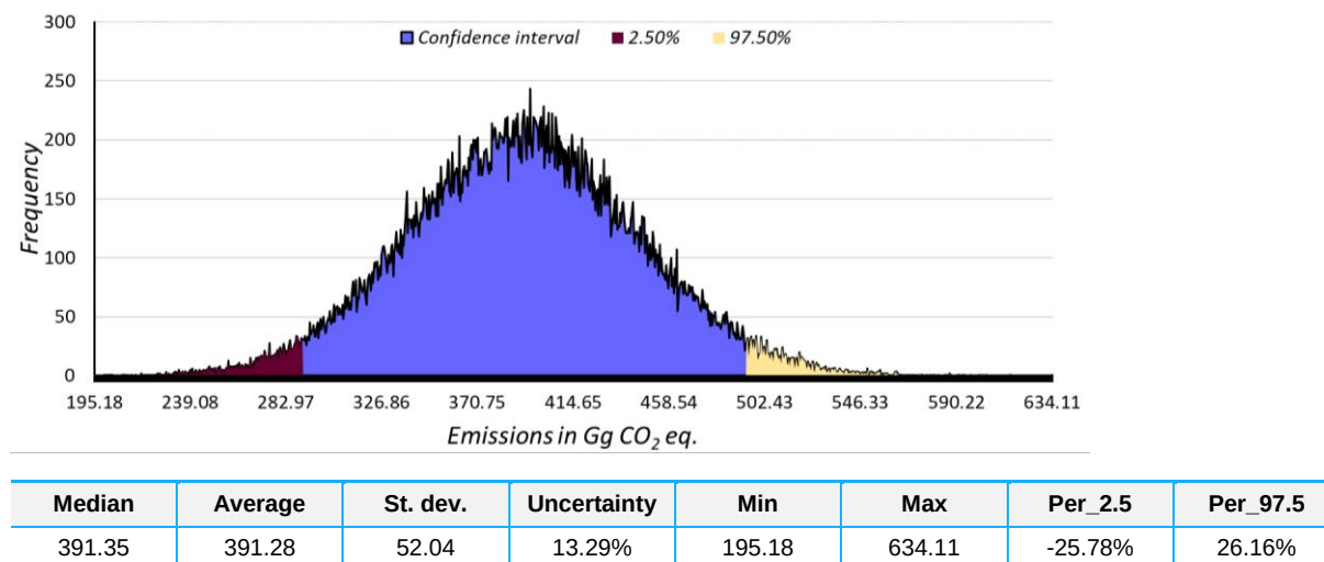
Figure 4.17: Probability density function for 2.B.8.b (t of CO 2 eq.)
