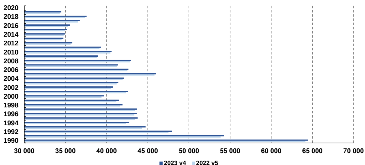
Figure 10.2: Comparison of the recalculated GHG emissions trend with LULUCF and with indirect emissions in 2022 (AR4) and 2023 (AR5) submissions for 1990 – 2020 in Gg of CO 2 eq.
