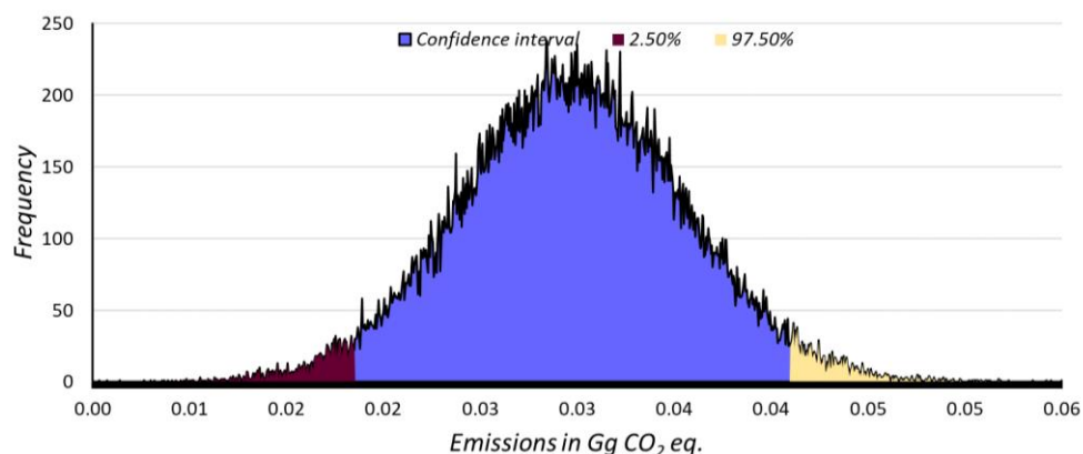
Figure 4.26: Probability density function for 2.C.5 (t of CO 2 eq.)
