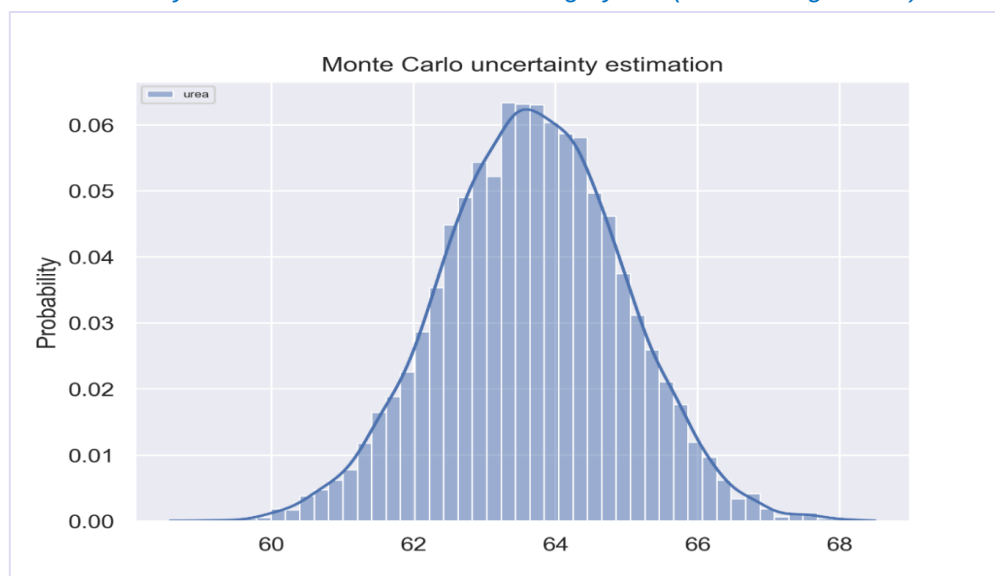
Figure 5.14: Probability distribution function for the category 3.H (x-axis in Gg of CO 2 )
