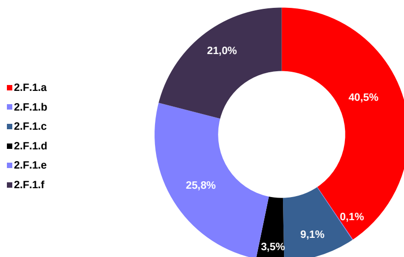
Figure 4.33: The share of individual subcategories within the category 2.F.1 in 2021
