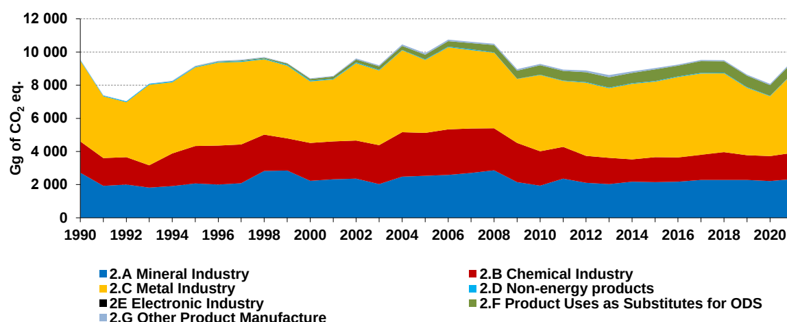
Figure 4.3: Trend of emissions in the IPPU sector according to the categories in 1990 – 2021
