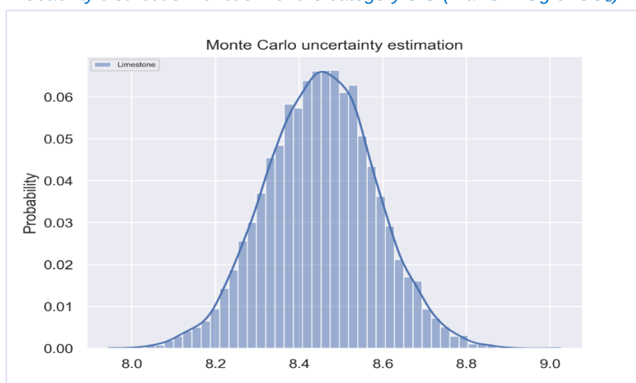
Figure 5.13: Probability distribution function for the category 3.G (x-axis in Gg of CO 2 )
