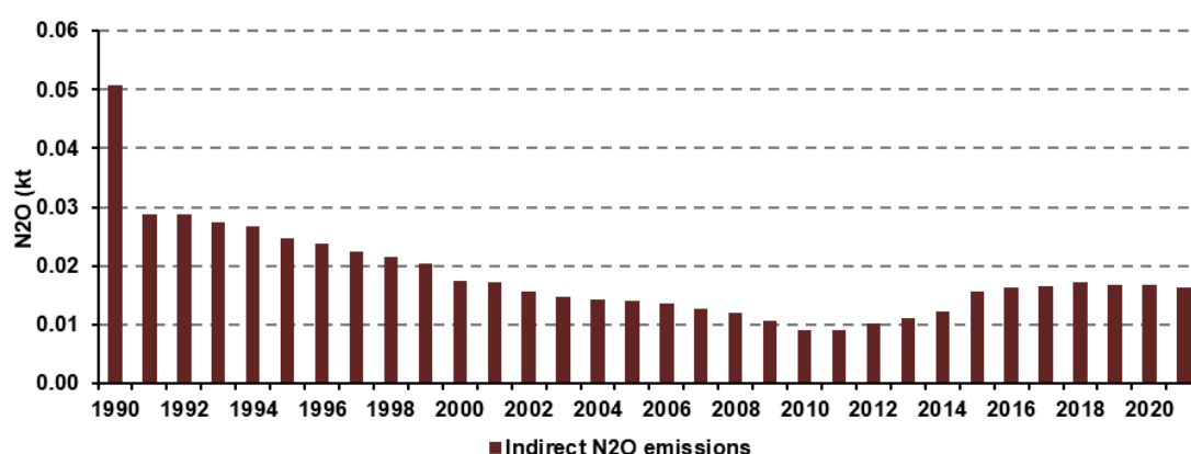
Figure 6.25: Summary of indirect N 2 O emissions (kt) from managed soils in 1990 – 2021
