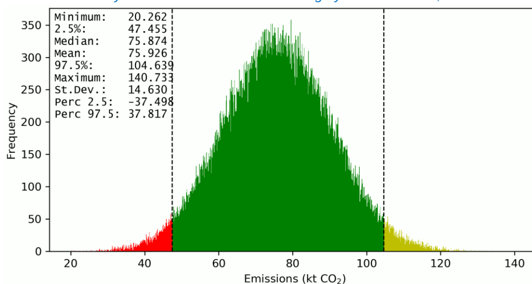
Figure A6.2.5: Probability distribution function for the category 4.F Other Land, 2021
