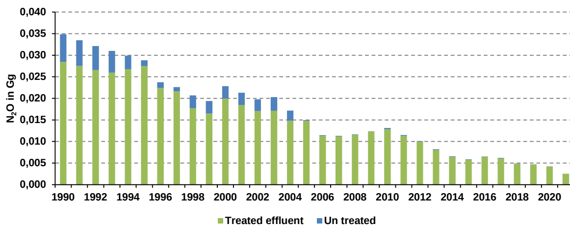
Figure 7.12: Distribution of the N 2 O emissions (in Gg) from the industrial wastewater
