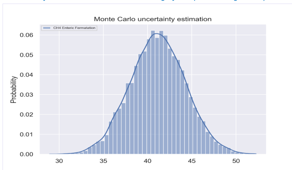
Figure 5.9: Probability distribution function for the category 3.A (x-axis in Gg of CH 4 )
