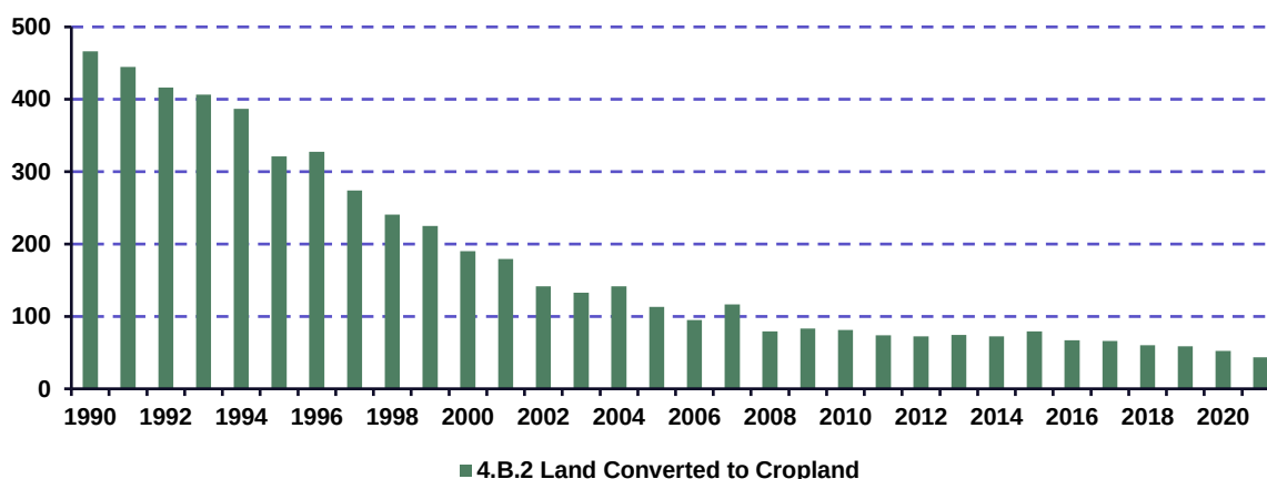
Figure 6.15: Summary of CO 2 emissions (kt) in L-CL subcategory in 1990 – 2021
