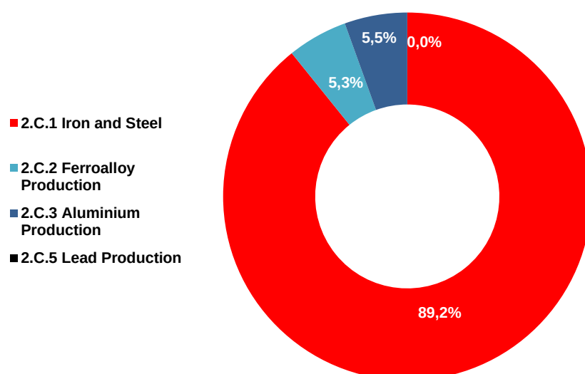
Figure 4.21: The share in GHG emissions in the category 2.C by subcategories in 2021
