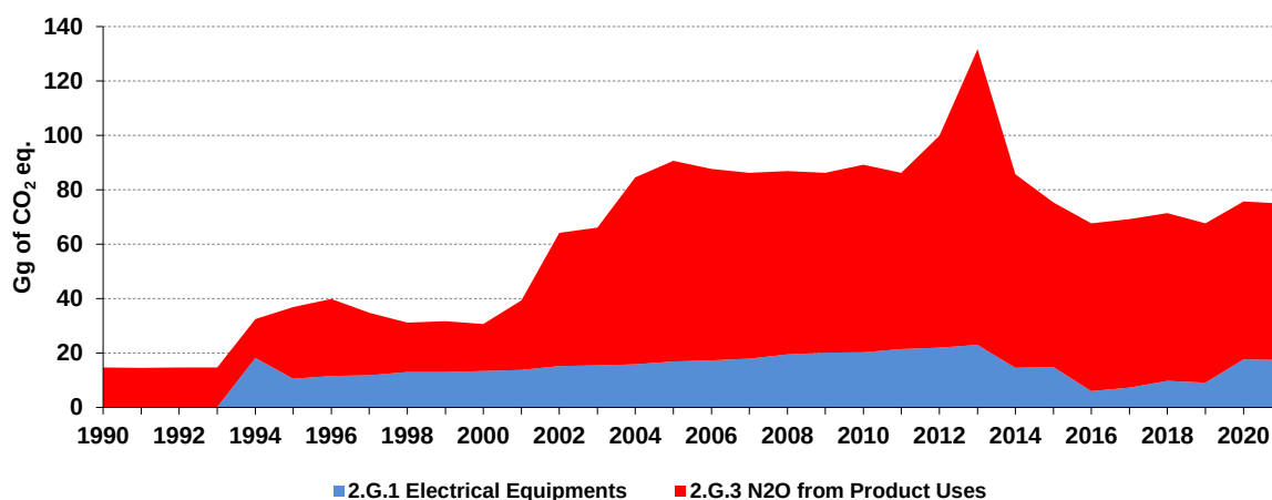
Figure 4.39: The trend of individual subcategories in the category 2.G in 1990 – 2021
