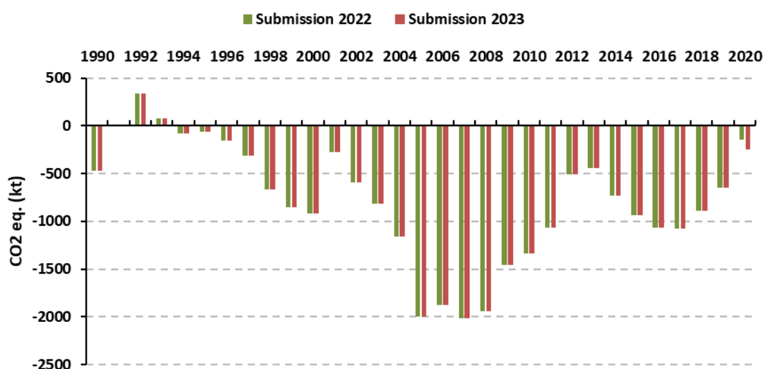
Figure 6.5: Comparison of CO 2 eq. (kt) in the 2022 and 2023 submissions for Harvested wood products
