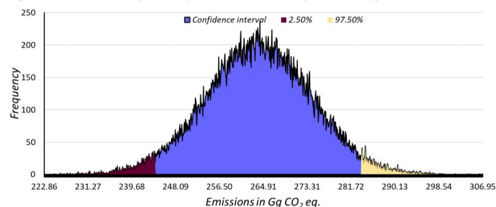
Figure 4.25: Probability density function for 2.C.3 (t of CO 2 eq.)
