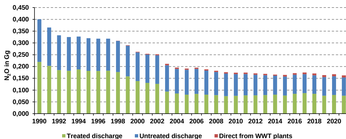
Figure 7.12: Distribution of the N 2 O emissions (in Gg) from the industrial wastewater
