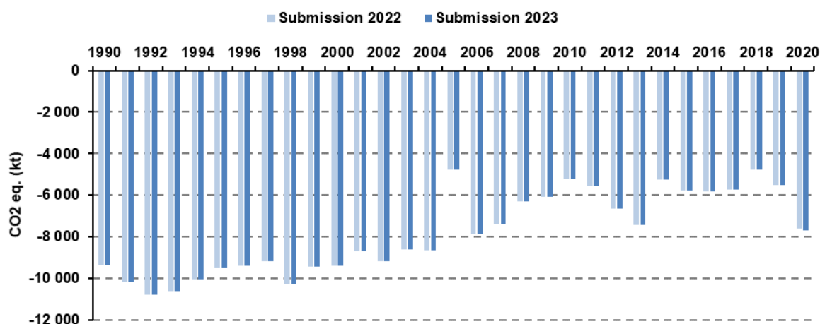
Figure 6.5: Comparison of CO 2 eq. (kt) in the 2022 and 2023 submissions for Harvested wood products
