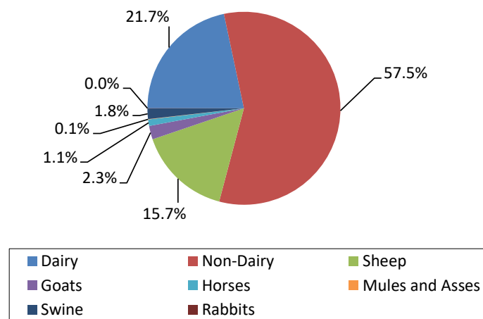
Figure 5-7: Relative importance of CH 4 emissions from enteric fermentation per each animal species, in 2021
