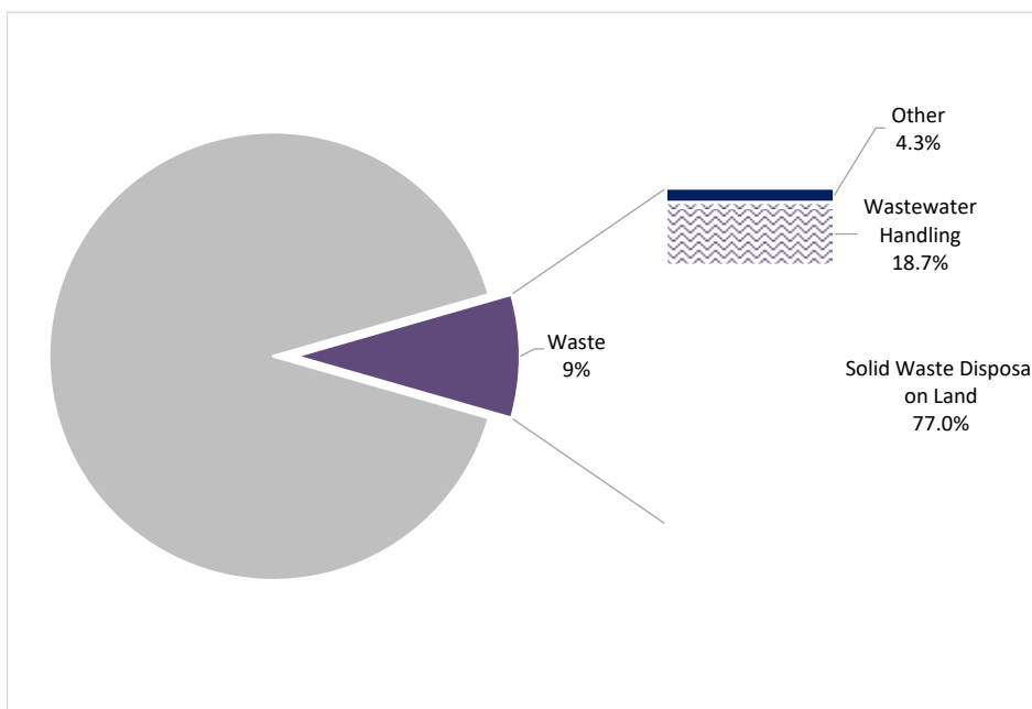
Figure 7-1: Greenhouse gas emissions from the waste sector in 2021
