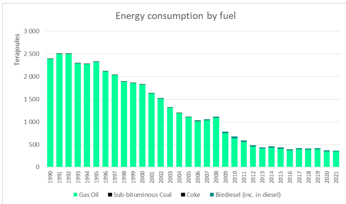
Figure 3-42: Consumption of fuels in the railway transport sector.
