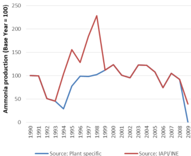
Figure 4-28: Ammonia production data – comparison of approaches
