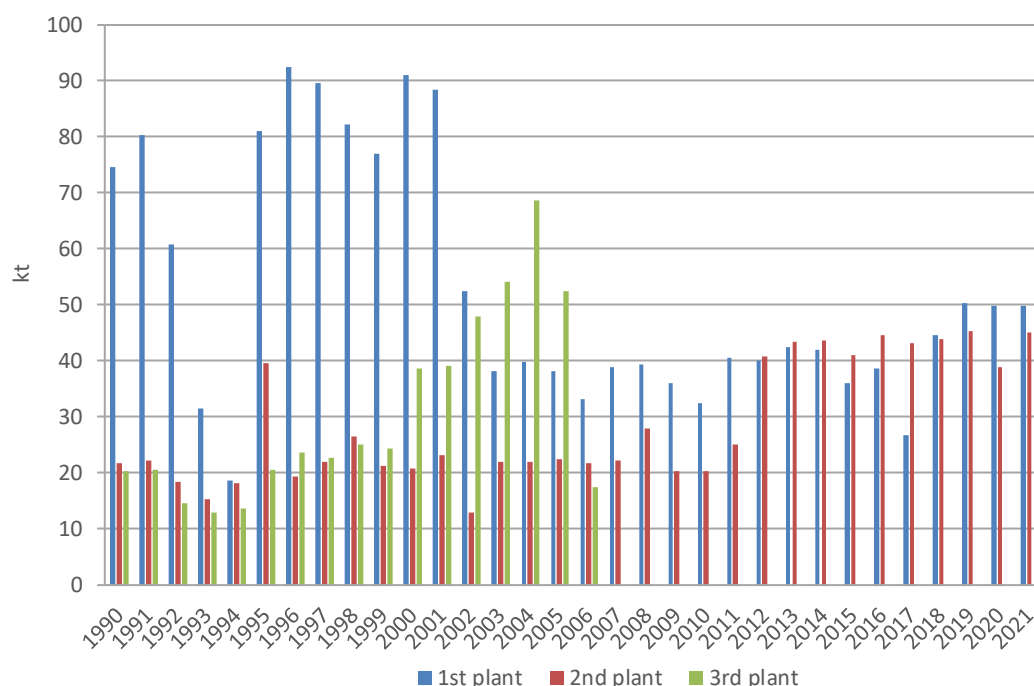
Figure 4-8. Glass production
