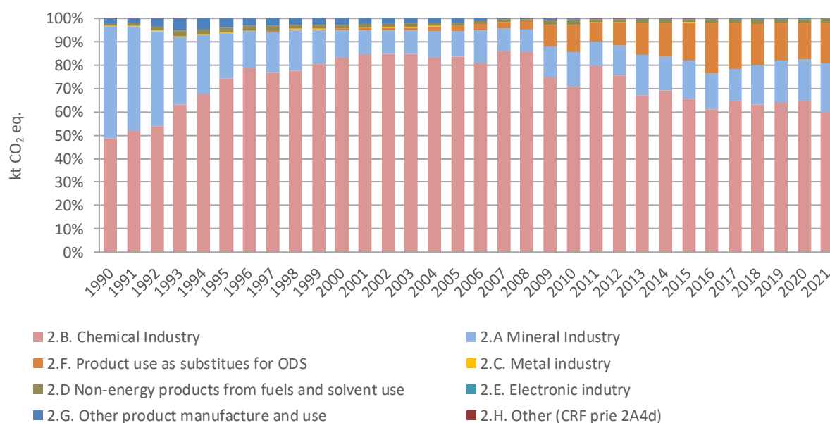
Figure 4-3. GHG emissions from industrial processes
