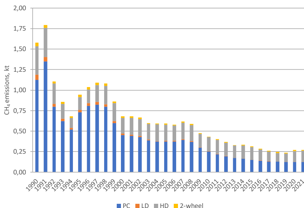
Figure 3-38. CH 4 emissions in Road transport
