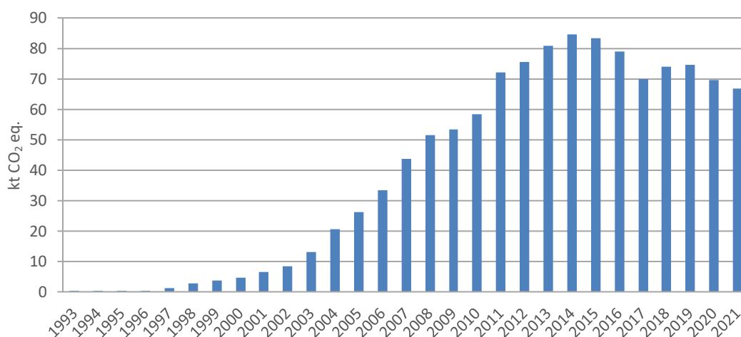
Figure 4-31. HFCs emissions from refrigerated road vehicles
