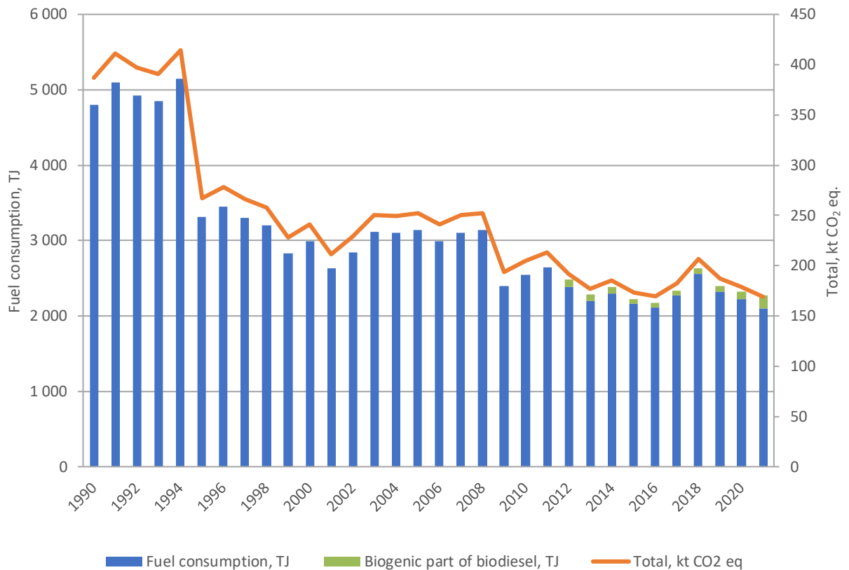
Figure 3-49. Trend of total GHG emissions and fuel consumption in Railways sector
