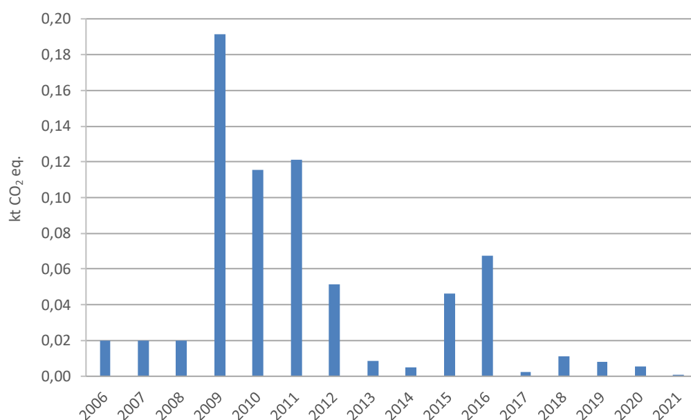
Figure 4-32. HFCs emissions from freight wagons
