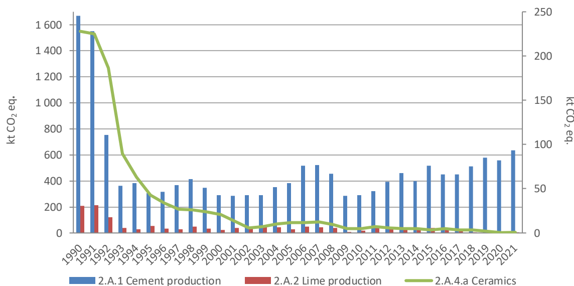
Figure 4-4. Greenhouse gas emission from mineral industry: cement production, lime production and ceramics
