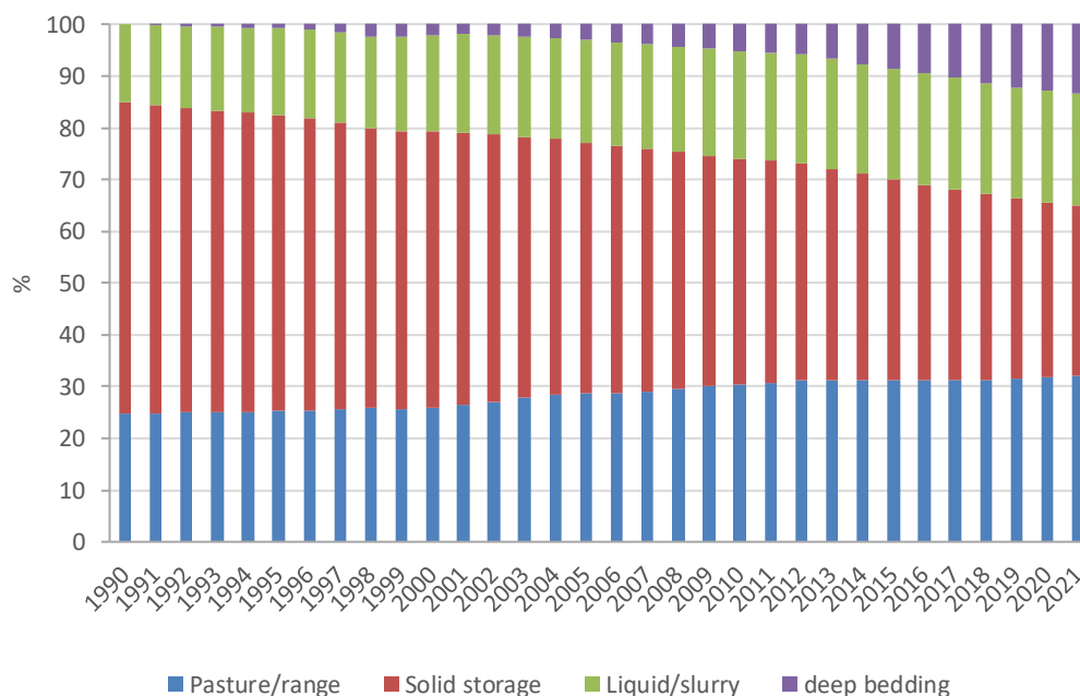
Figure 5-3. Data on manure management systems for dairy cattle
