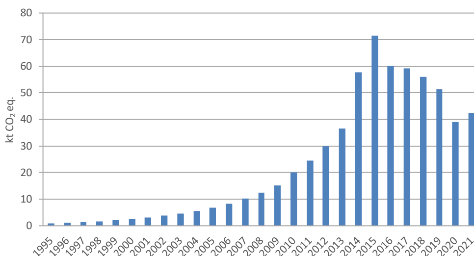
Figure 4-27. HFCs emissions from industrial refrigeration
