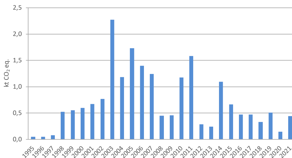
Figure 4-41. SF 6 emissions from electrical equipment
