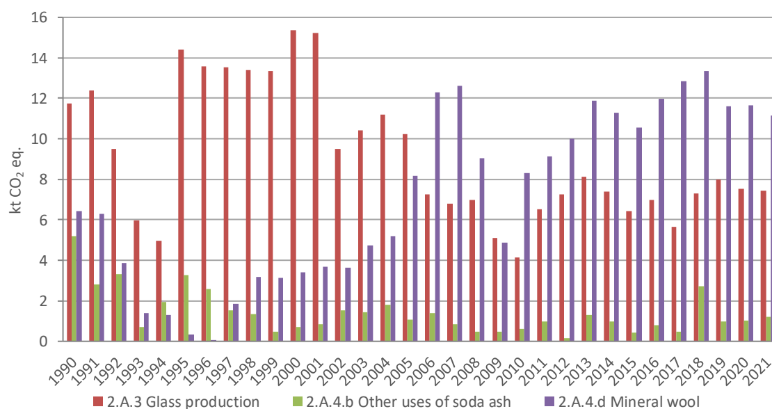
Figure 4-5. Greenhouse gas emissions from mineral industry: glass production, soda ash use and mineral wool production
