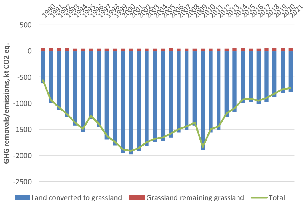
Figure 6-24. GHG emissions and removals in grassland in 1990-2021, kt CO 2 eq.
