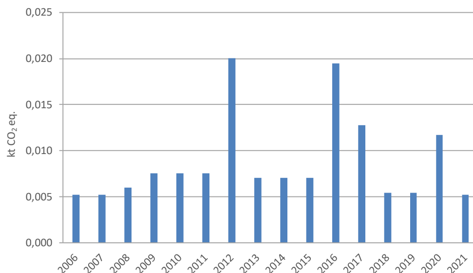
Figure 4-35. HFCs emissions from passenger carriages
