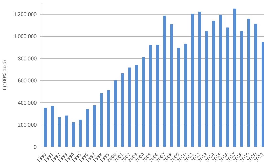
Figure 4-15. Nitric acid production
