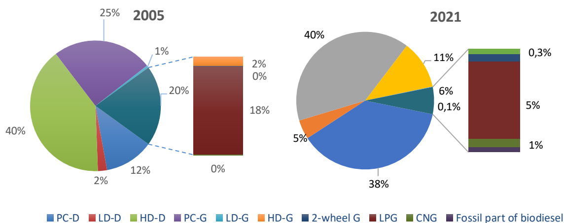
Figure 3-42. Fuel consumption share (TJ) per vehicle type and fuel type for road transport in 2005 and 2021. PC-D – diesel passenger cars, LD-D – diesel light-duty vehicles, HD-D – diesel heavy-duty vehicles, PC-G – gasoline passenger cars, LD-G – gasoline passenger cars, HD-G – gasoline heavy-duty vehicles, 2-wheel G – gasoline 2-wheelers, LPG – LPG passenger cars, CNG – CNG passenger cars.
