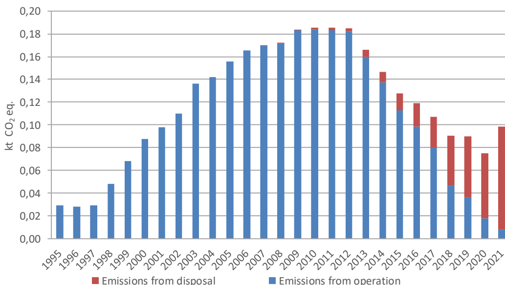
Figure 4-30. HFCs emissions from domestic freezers
