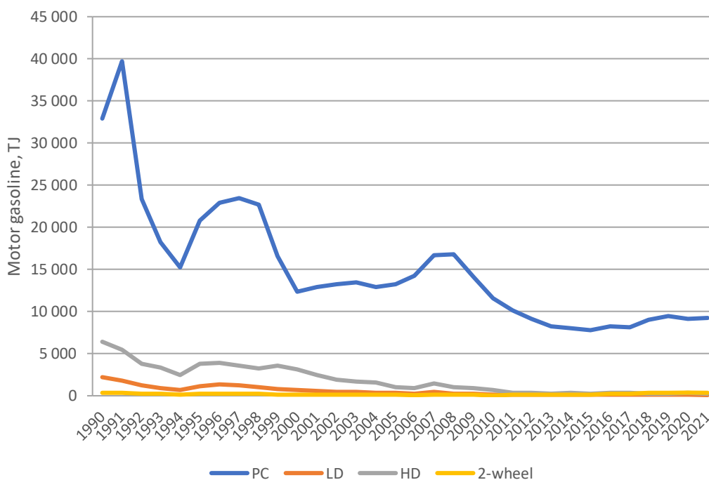
Figure 3-40. Gasoline fuel consumption per vehicle type for road transport
