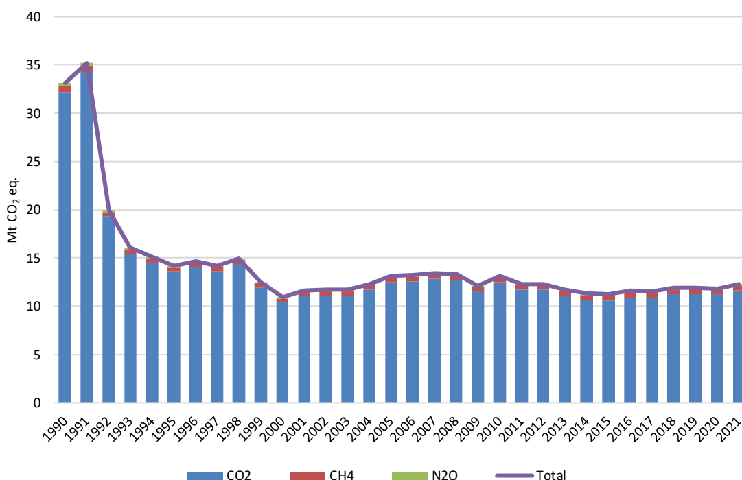
Figure 3-11. Trends of total GHG emissions from the Energy Sector (CRF 1)
