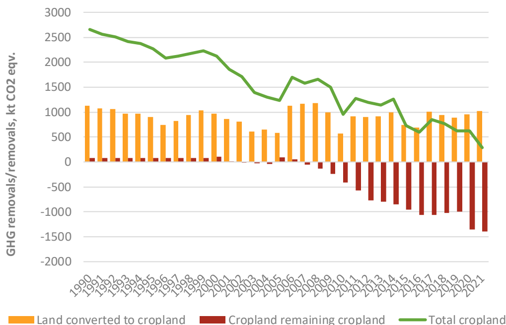
Figure 6-20. Greenhouse gas emissions in cropland, kt CO 2 eq.
