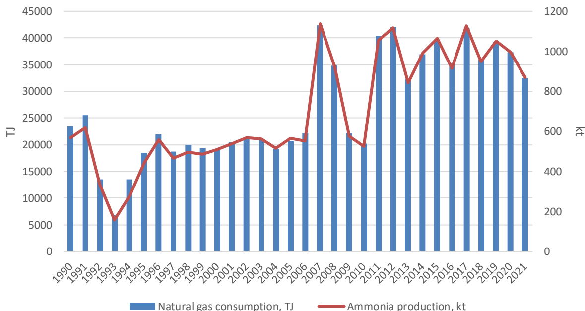
Figure 4-14. Ammonia production and natural gas consumption
