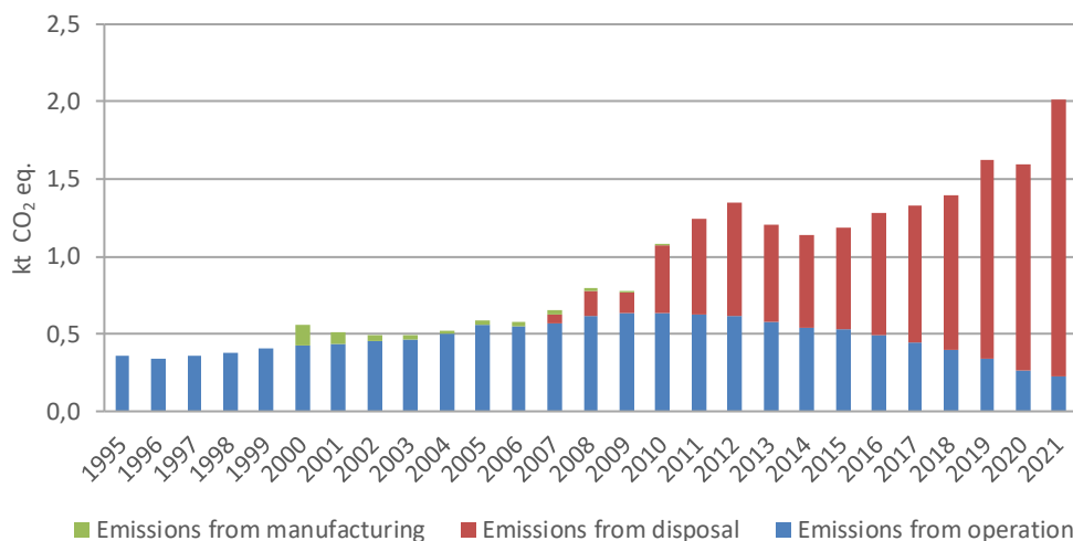
Figure 4-29. HFCs emissions from domestic refrigerators
