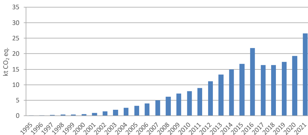
Figure 4-36. HFCs emissions from stationary air conditioning
