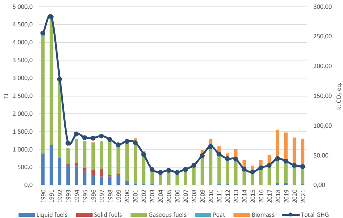
Figure 3-22. Tendencies of fuel consumption and total GHG emissions in Pulp, Paper and Print industries (1.A.2.d)
