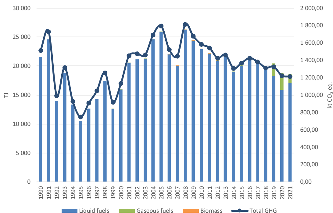
Figure 3-18. Tendencies of fuel consumed and total GHG emissions in Petroleum Refinery (1.A.1.b)
