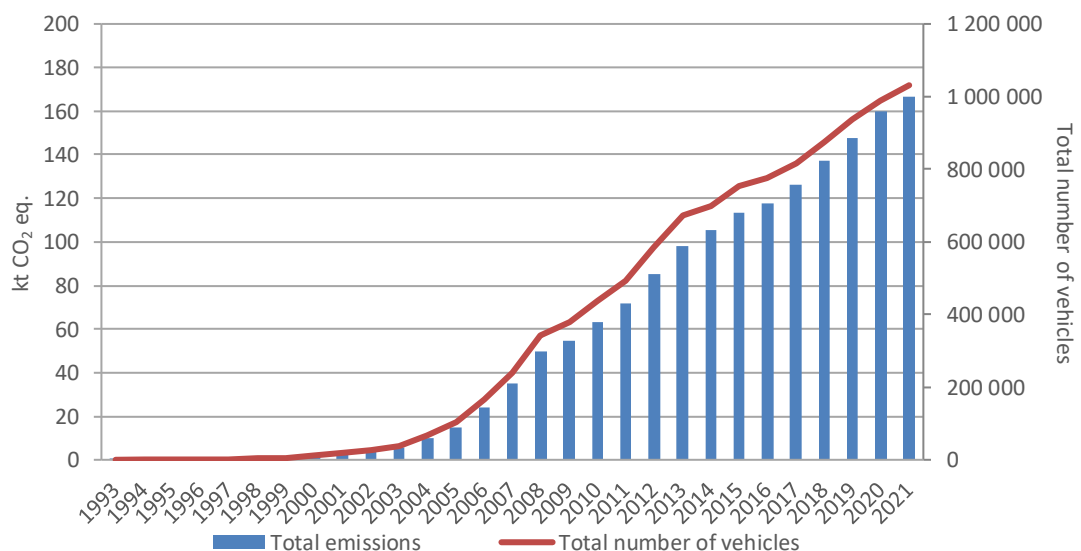
Figure 4-34. HFCs emissions from vehicles with air conditioning
