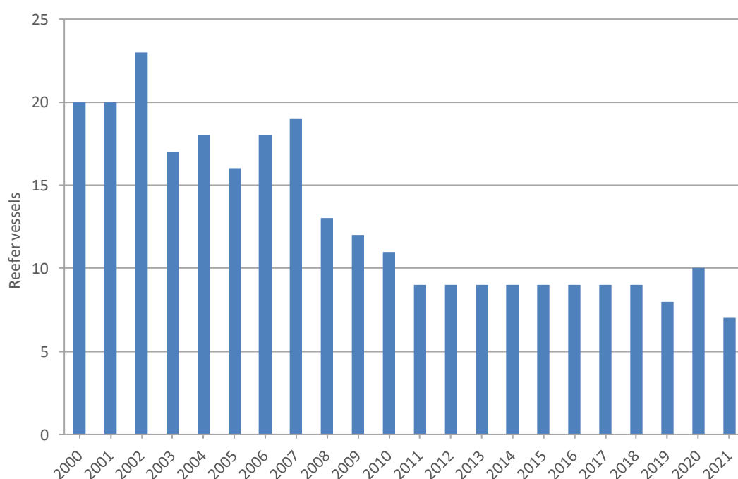
Figure 4-33. Reefer vessels registered in Lithuania
