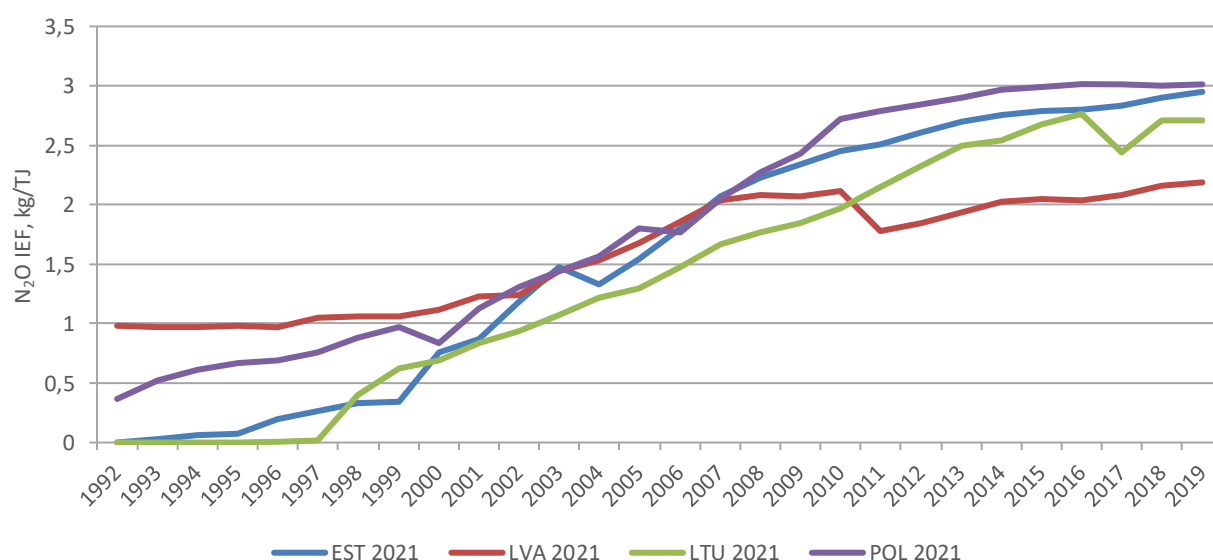
Figure 3-44. N 2 O IEF values provided by Lithuania and the neighbouring countries for diesel Passenger Cars
