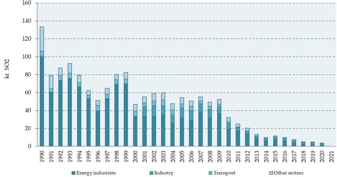
Figure 3.1-11: SO 2 emissions from Energy sector in the period 1990-2021
