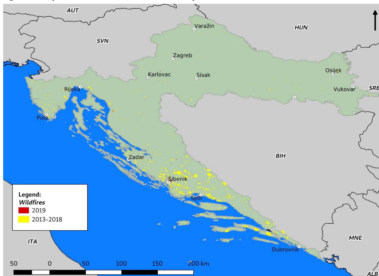
Figure 6.15-4: Spatial distribution of forest fires in Croatia for period 2013-2019
