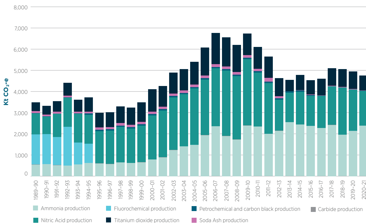
Figure 4.11 Emissions from the chemical industry, Australia, 1989–90 to 2020–21, kt CO 2 -e
