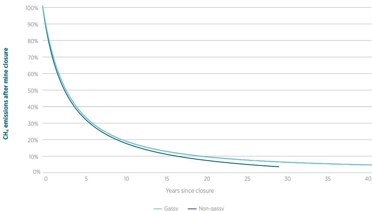
Figure 3.28 CH 4 decay curves for gassy and non-gassy Australian decommissioned coal mines
