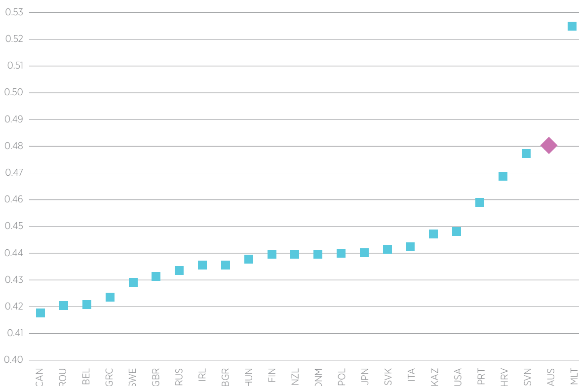
Figure 4.10 Other Process Uses of Carbonates implied emission factors for Annex I countries (2022 submission) and Australia (2023 submission), tonnes of CO 2 per tonne of carbonate
