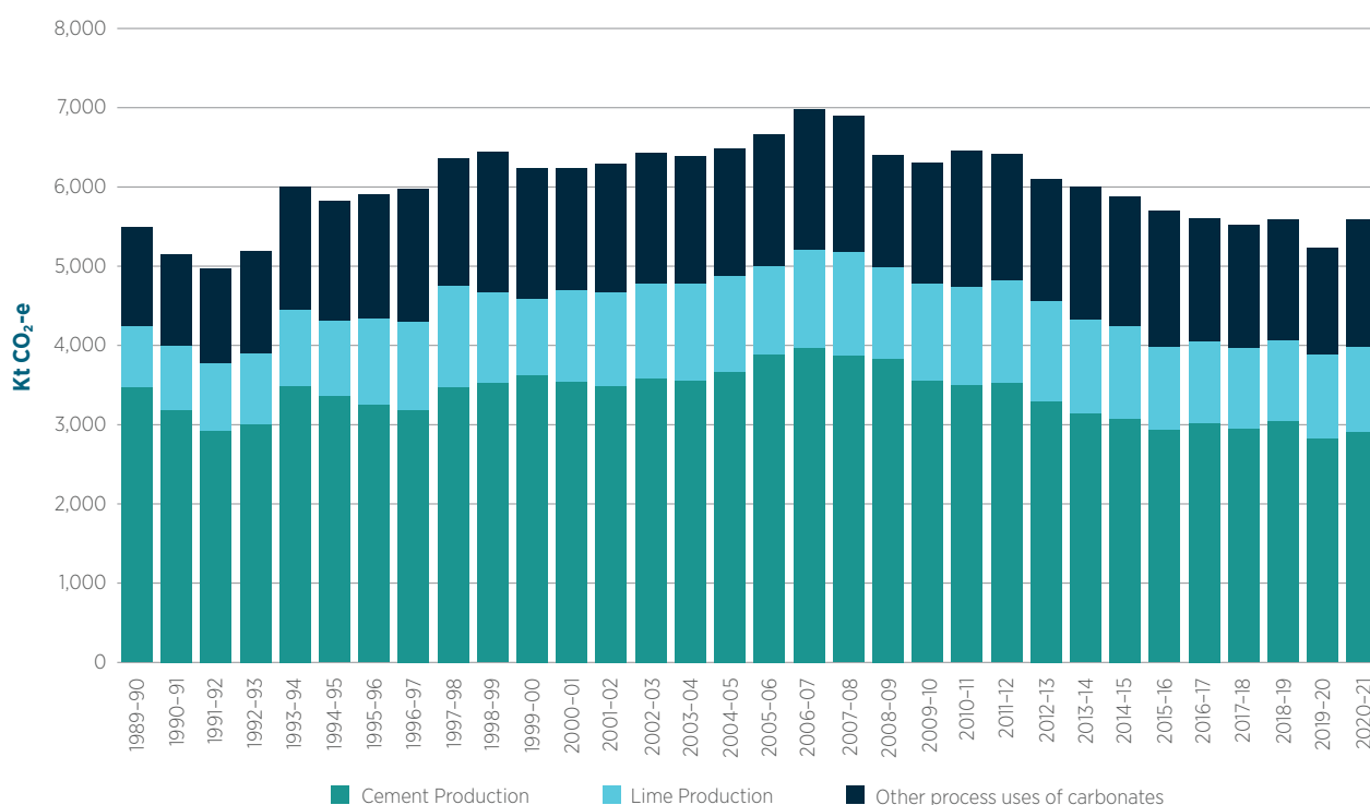
Figure 4.6 Emissions from the mineral industry, Australia, 1989–90 to 2020–21, kt CO 2 -e
