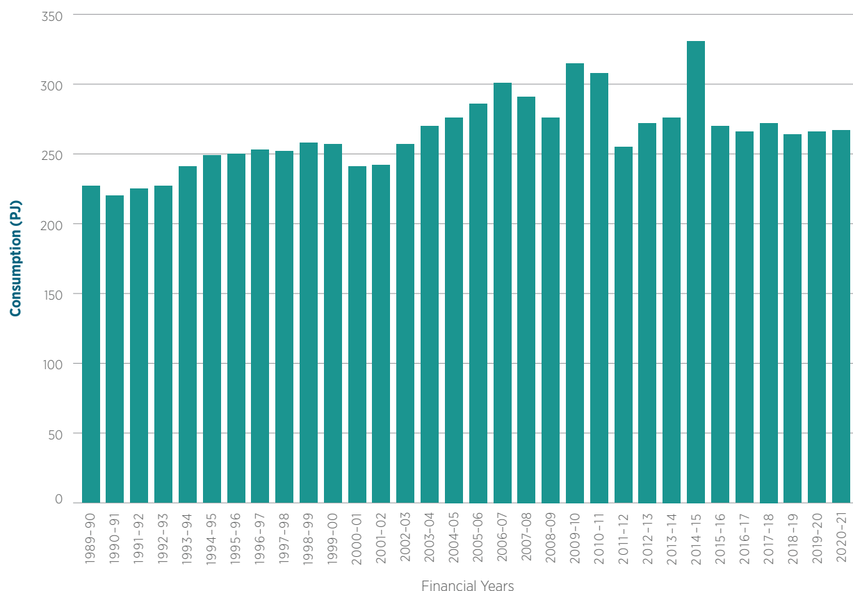
Figure 3.11 Consumption of non-energy uses of energy products, PJ
