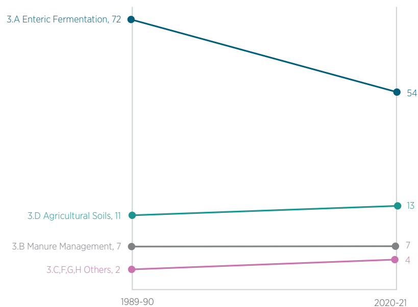
Figure 5.3 Slope chart comparing emissions by agriculture sub-sector in 1989-90 and 2020-21, Australia, Mt CO 2 -e
