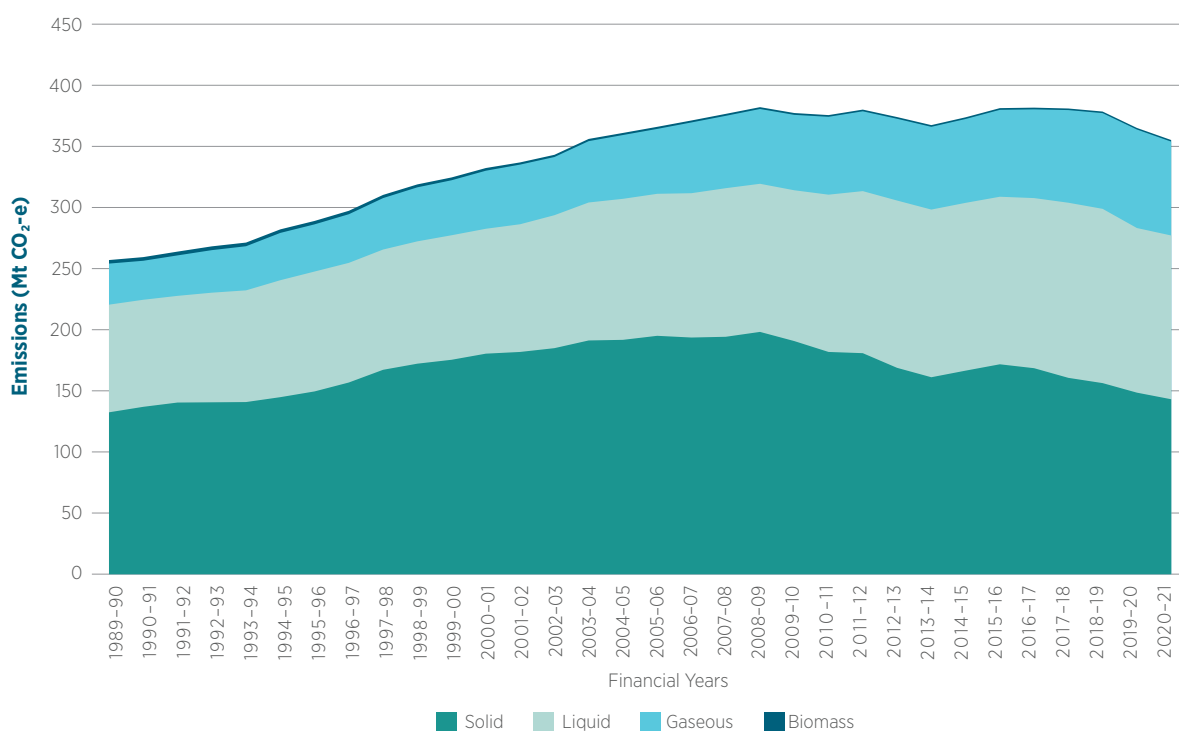
Figure 3.5 Solid, liquid, and gaseous fuel combustion has increased, and biomass combustion has decreased, since 1989–90
