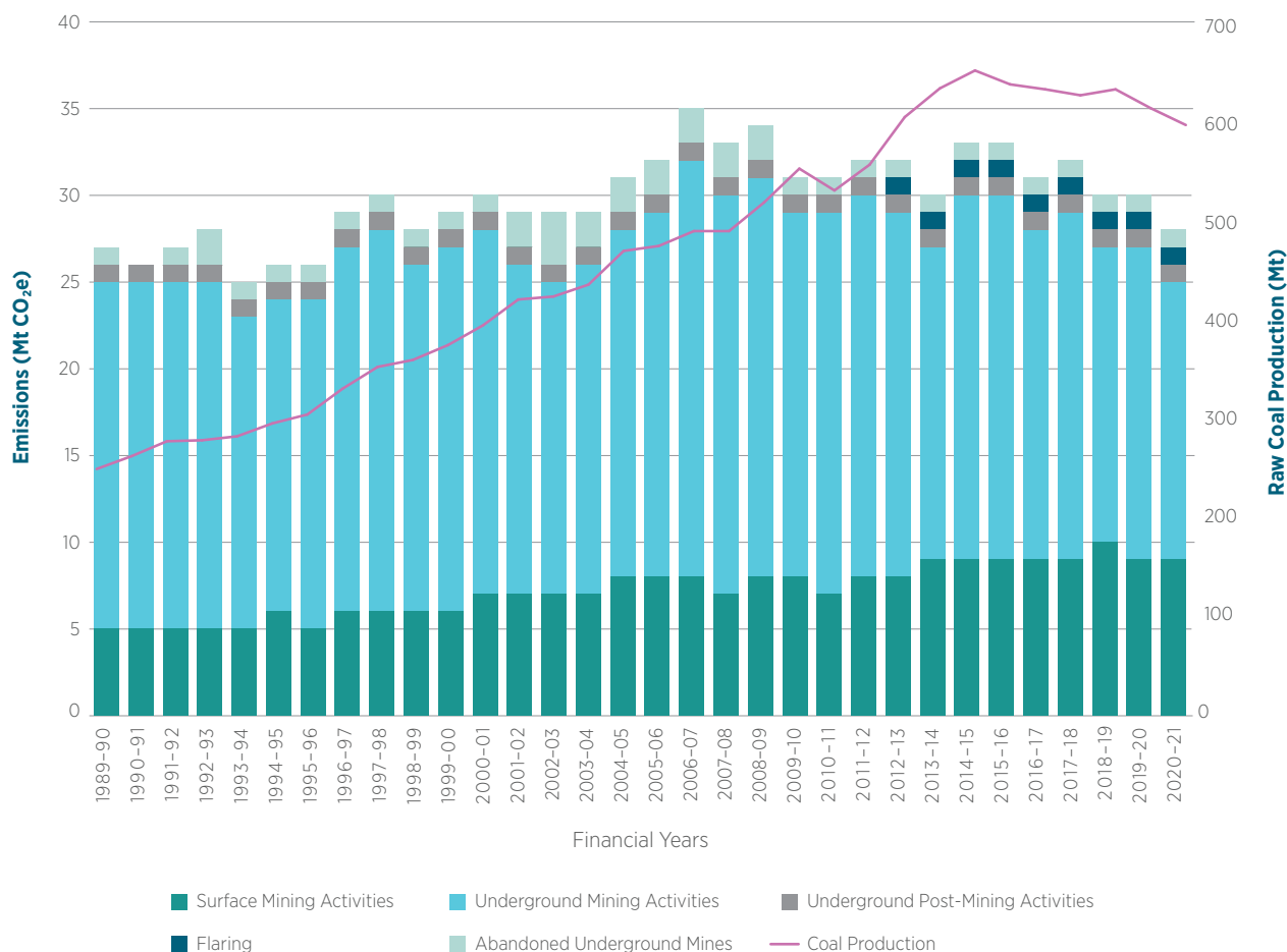
Figure 3.23 Fugitive CO 2 -e emissions and coal production from coal mining activities, 1989–90 to 2020–21
