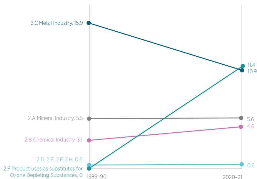
Figure 4.5 Slope chart comparing emissions by IPPU sub-sector in 1989–90 and 2020–21, Australia, Mt CO 2 -e
