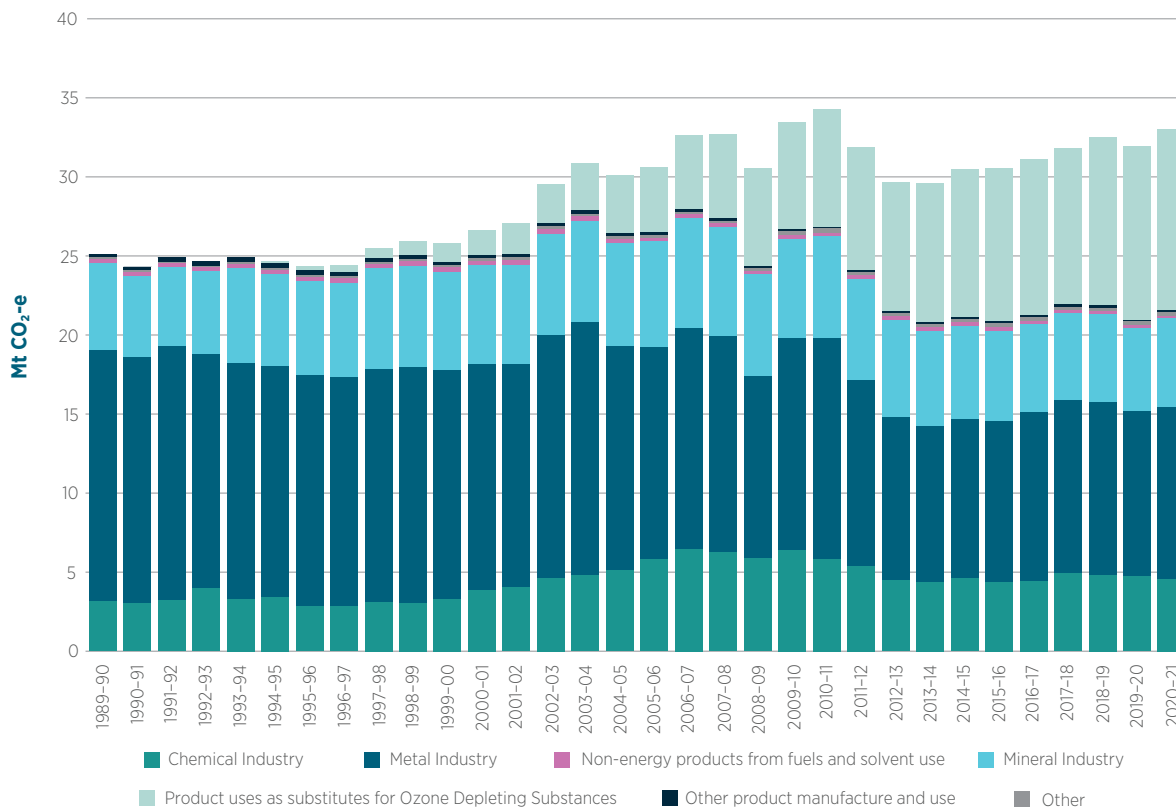
Figure 4.3 Industrial Process and Product Use emissions by subsector, 1989–20 to 2020–21
