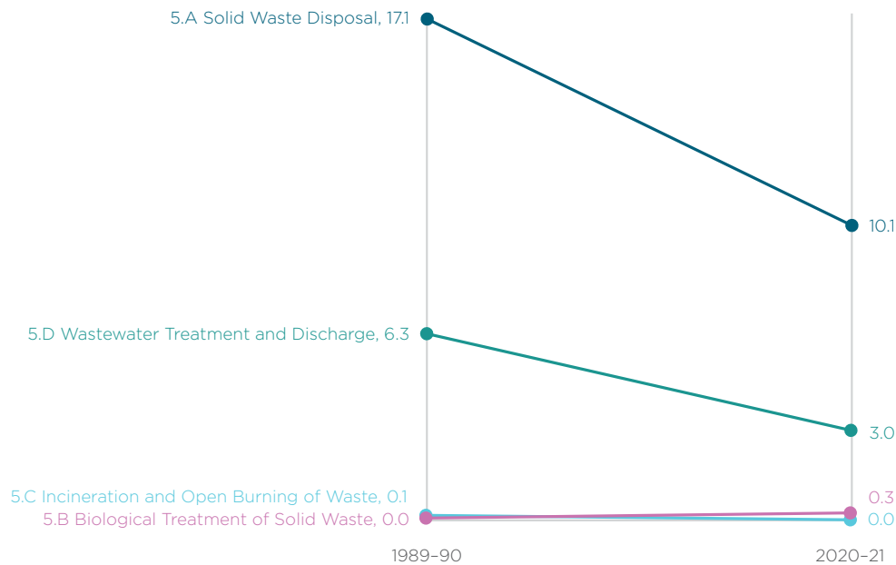
Figure 7.3 Slope chart comparing emissions by waste sub-sector in 1989-90 and 2020-21, Australia, Mt CO 2 -e
