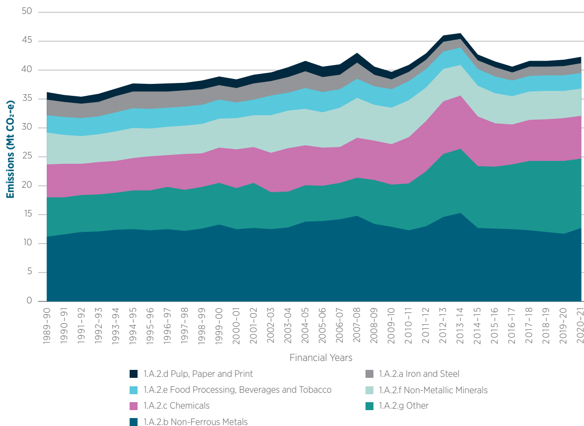
Figure 3.14 Emissions from the manufacturing and construction industries by subsector
