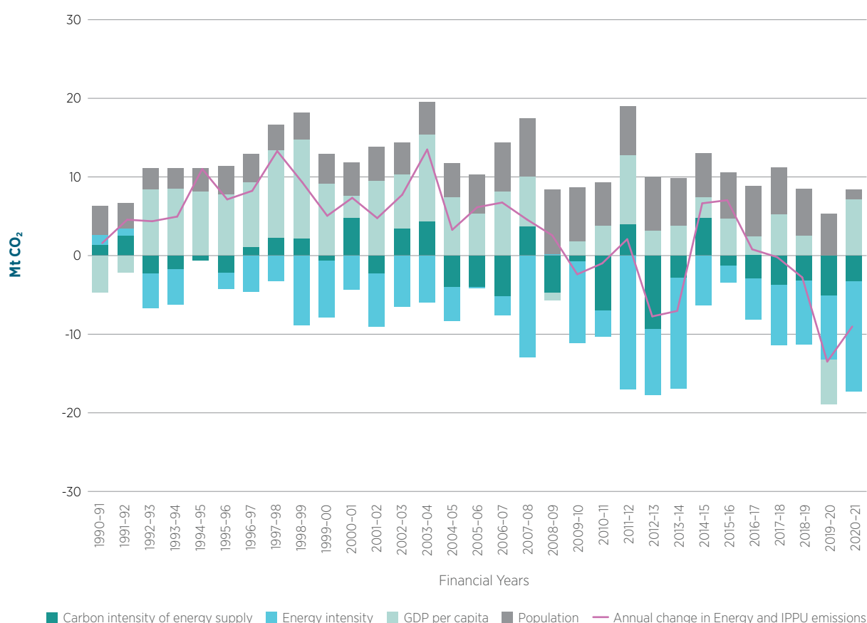
Figure 2.11 Annual change in CO 2 emissions from fuel combustion and IPPU from underlying drivers, Australia, 1990–91 to 2020–21, Mt CO 2
