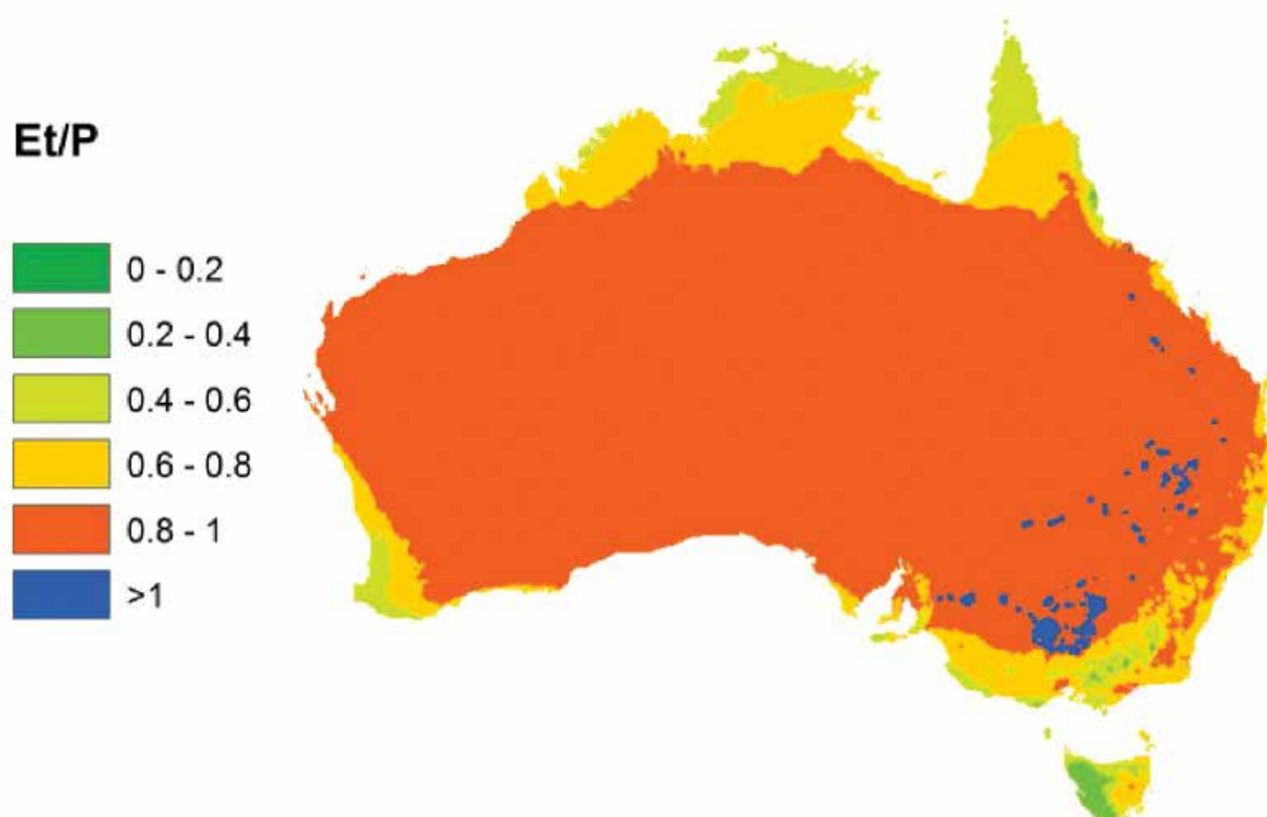
Figure 5.12 The ratio of mean annual evapotranspiration to annual precipitation (Et/P)
