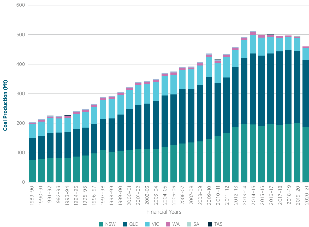
Figure 3.25 Coal production by State since 1989–90, Mt
