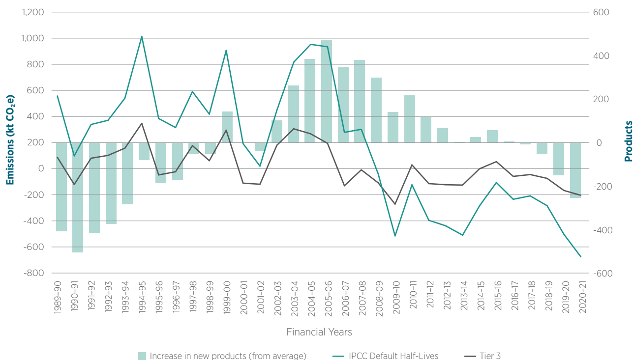
Figure 6.10.3 Comparison of the variability in the treatment of young products by the Tier 3 model and IPCC Tier 2 First Order Decay Model
