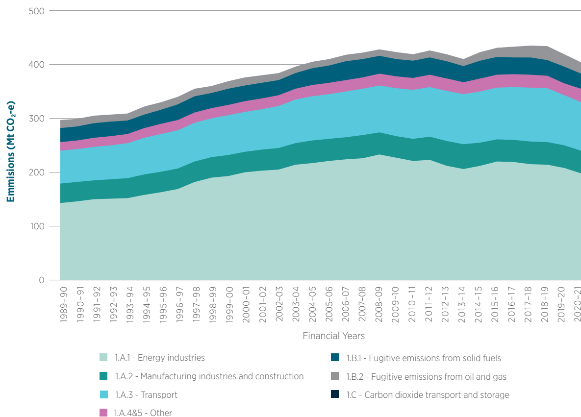
Figure 3.2 Energy emissions by subsector, 1989–90 to 2020–21
