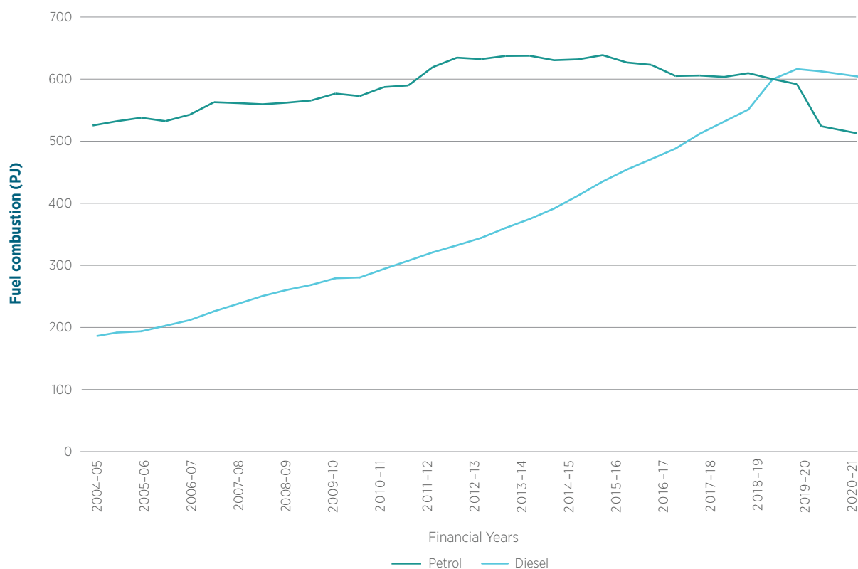
Figure 3.17 Energy consumption in road transport by fuel type, 2004-05 to 2020-21
