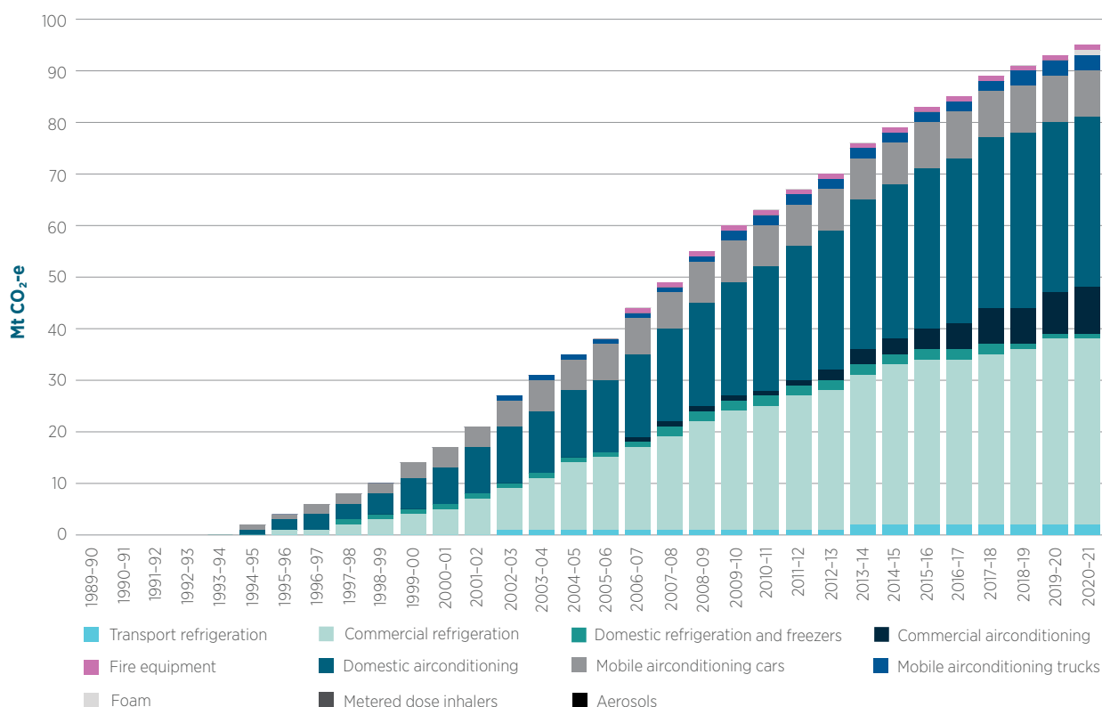
Figure 4.16 Growth in the bank of HF gas in operating equipment (Mt CO 2 -e)
