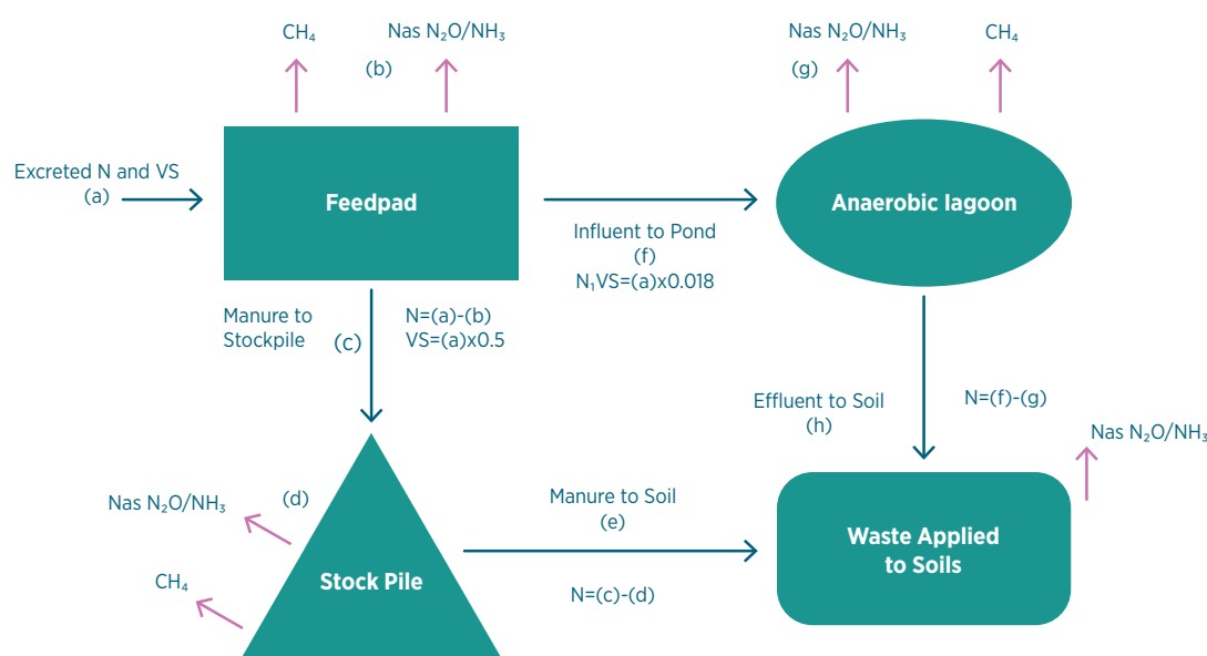
Figure 5.7 Mass flow method of estimating manure management emissions – feedlot cattle example
