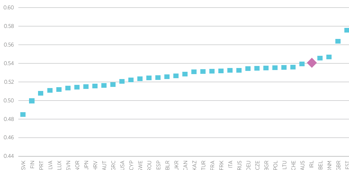
Figure 4.8 Cement production implied emission factors for Annex I countries (2022 submission) and Australia (2023 submission), tonnes of CO 2 per tonne of cement produced
