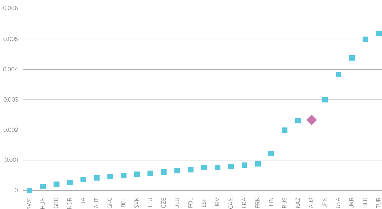
Figure 4.13 Nitric acid implied emission factors for Annex I countries (2022 submission) and Australia (2023 submission), tonnes of N 2 O per tonne of nitric acid produced
