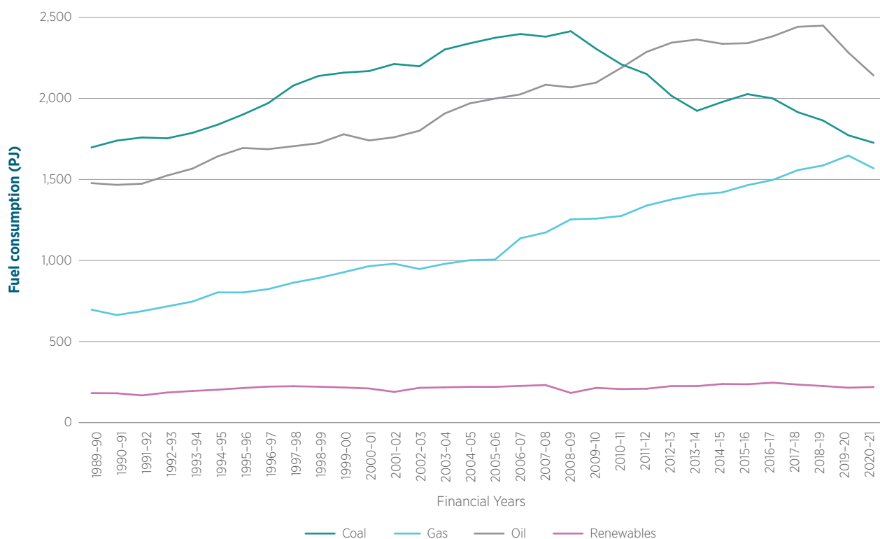
Figure 2.12 Energy consumption by fuel type, Australia, PJ
