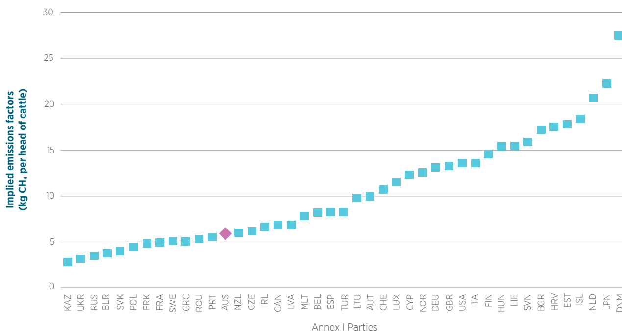
Figure 5.8 Cattle manure management implied emission factors for Annex I countries (2022 submission) and Australia (2023 submission), kg CH 4 per head per year
