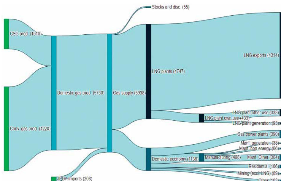
Figure 3.36 Australian natural gas energy flows, PJ, 2020–21
