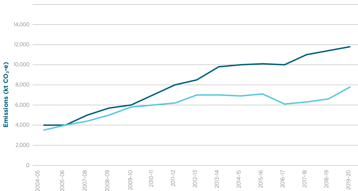
Figure 4.17 Comparison of Inventory HFC emission estimates with estimates derived from Cape Grim measurement data
