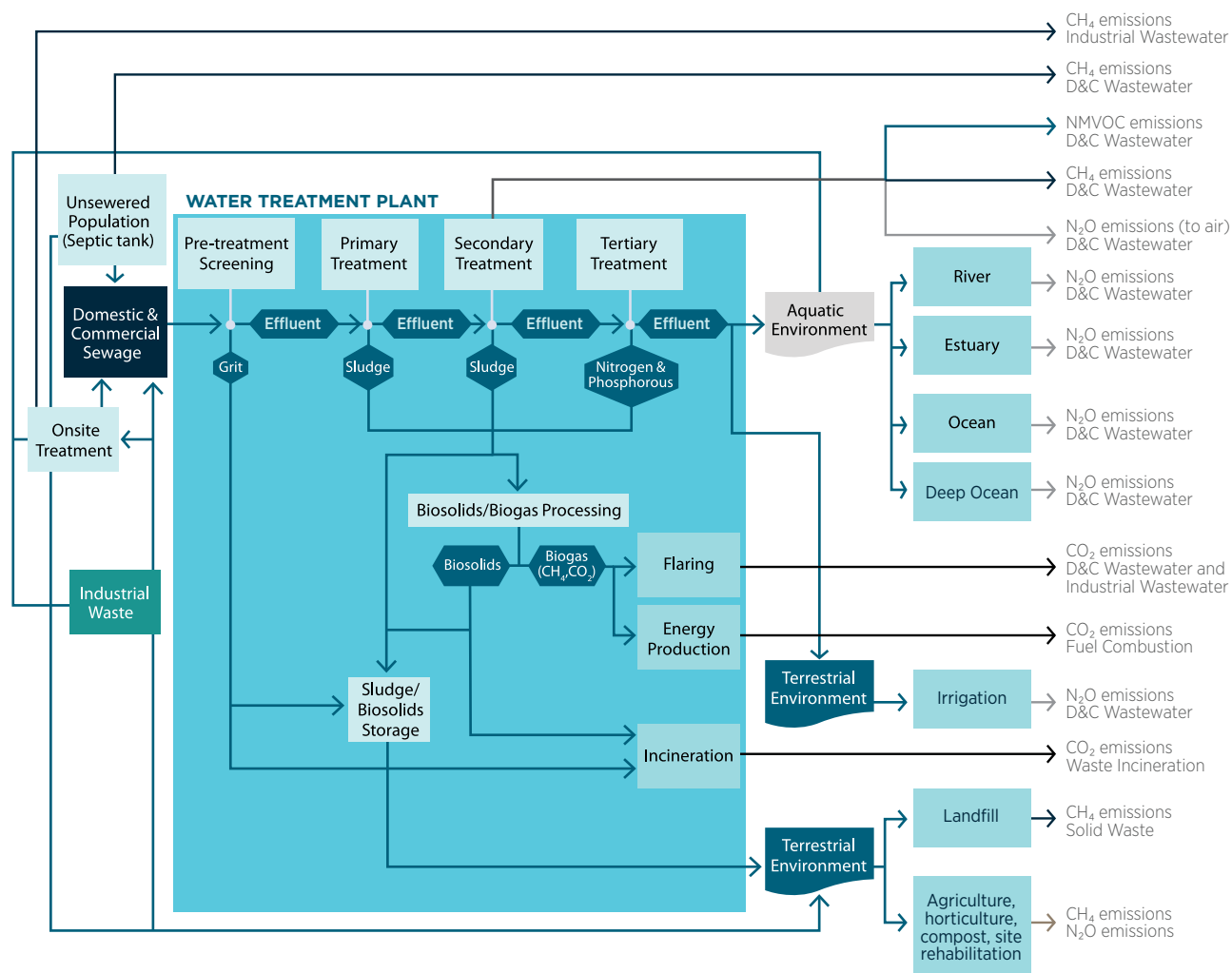
Figure 7.12 Pathways for Wastewater
