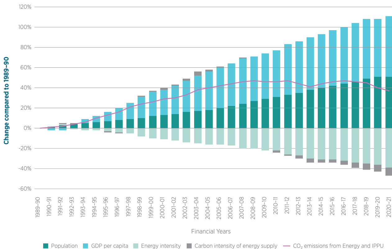
Figure 2.10 Growth in CO 2 emissions from fuel combustion and IPPU and underlying drivers, Australia, 1989–90 to 2020–21
