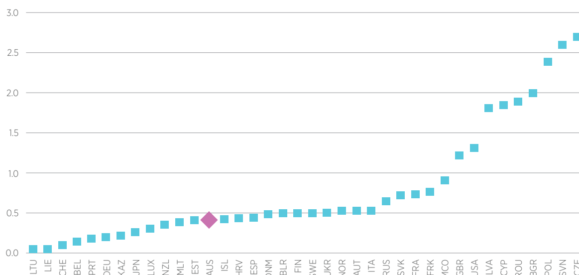
Figure 4.21 Product life emission factors for Annex I countries (2022 submission) and Australia (2023 submission), per cent
