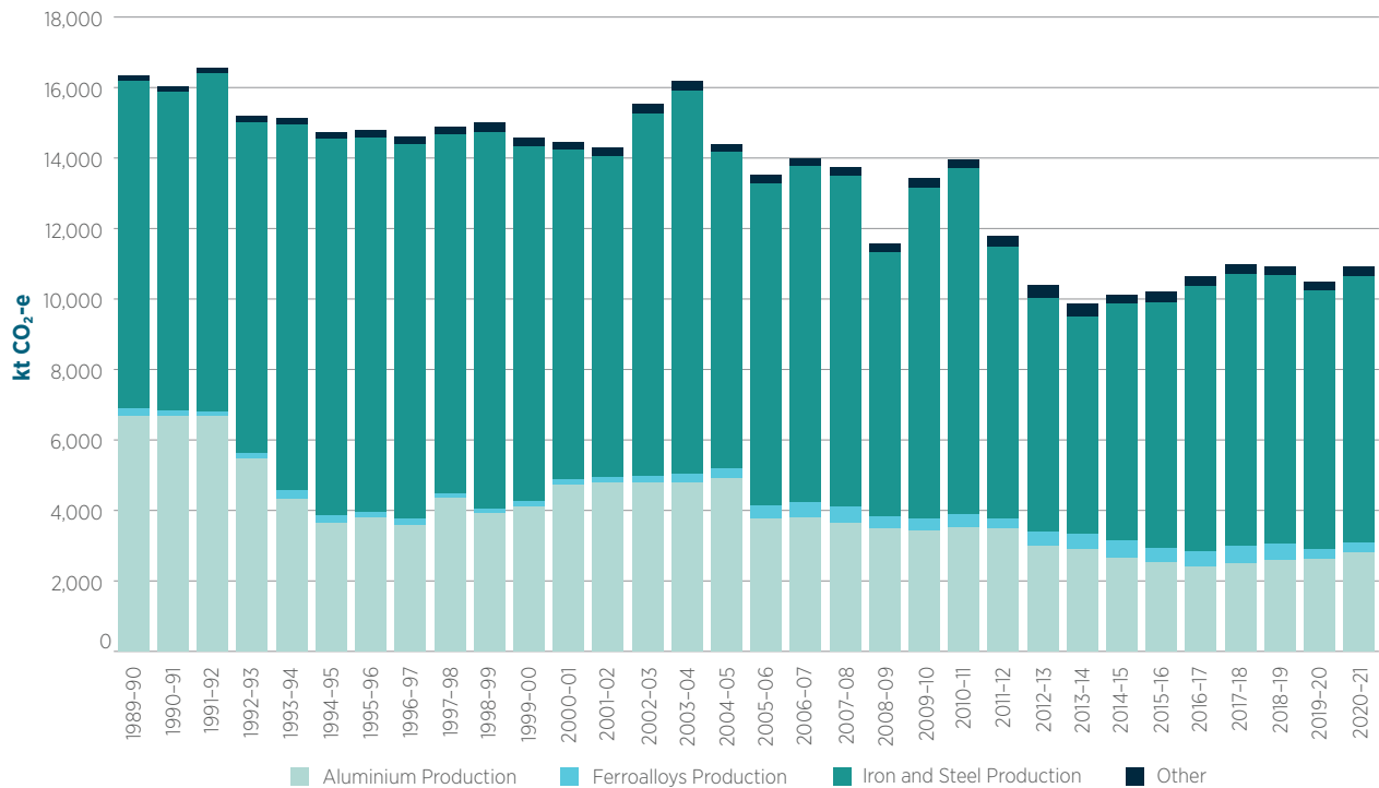
Figure 4.14 Emissions from the metal industry, Australia, 1989–90 to 2020–21, kt CO 2 -e
