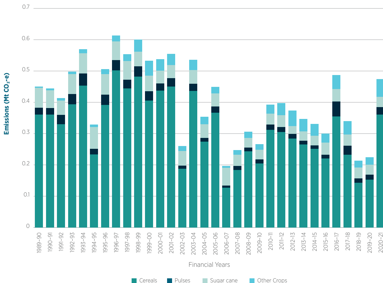
Figure 5.13 Emissions from field burning of agricultural residues, Australia, Mt CO 2 -e
