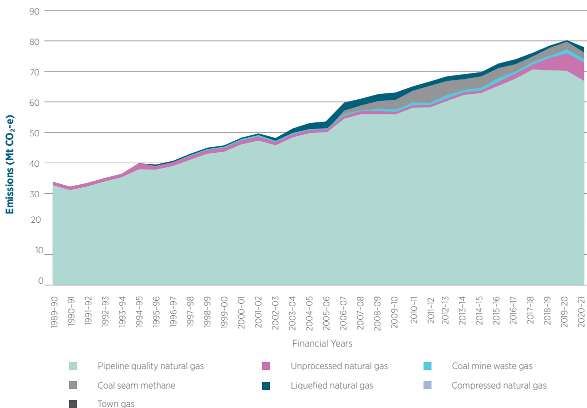
Figure 3.8 Emissions from gaseous fuel combustion, 1989–90 to 2020–21
