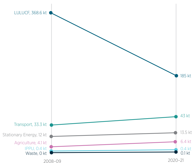
Figure 2.9 Slope chart comparing black carbon emissions by sector in 2008–09 and 2020–21, Australia, kt
