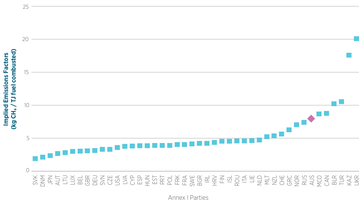
Figure 3.20 Implied emission factors from liquid fuel combustion for Annex I countries (2022 submission) and Australia (2023 submission), kg CH 4 per TJ combusted
