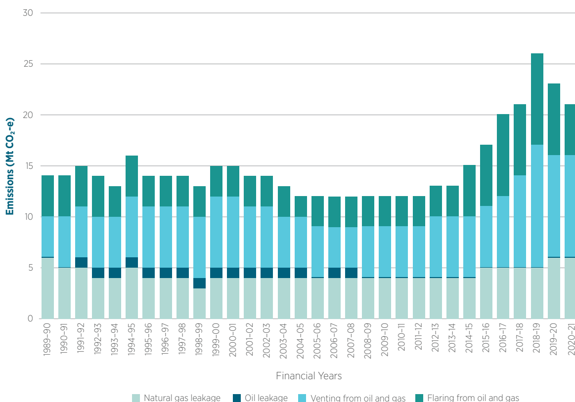
Figure 3.33 Fugitive CO 2 -e emissions from oil and gas, 1989–90 to 2020–21
