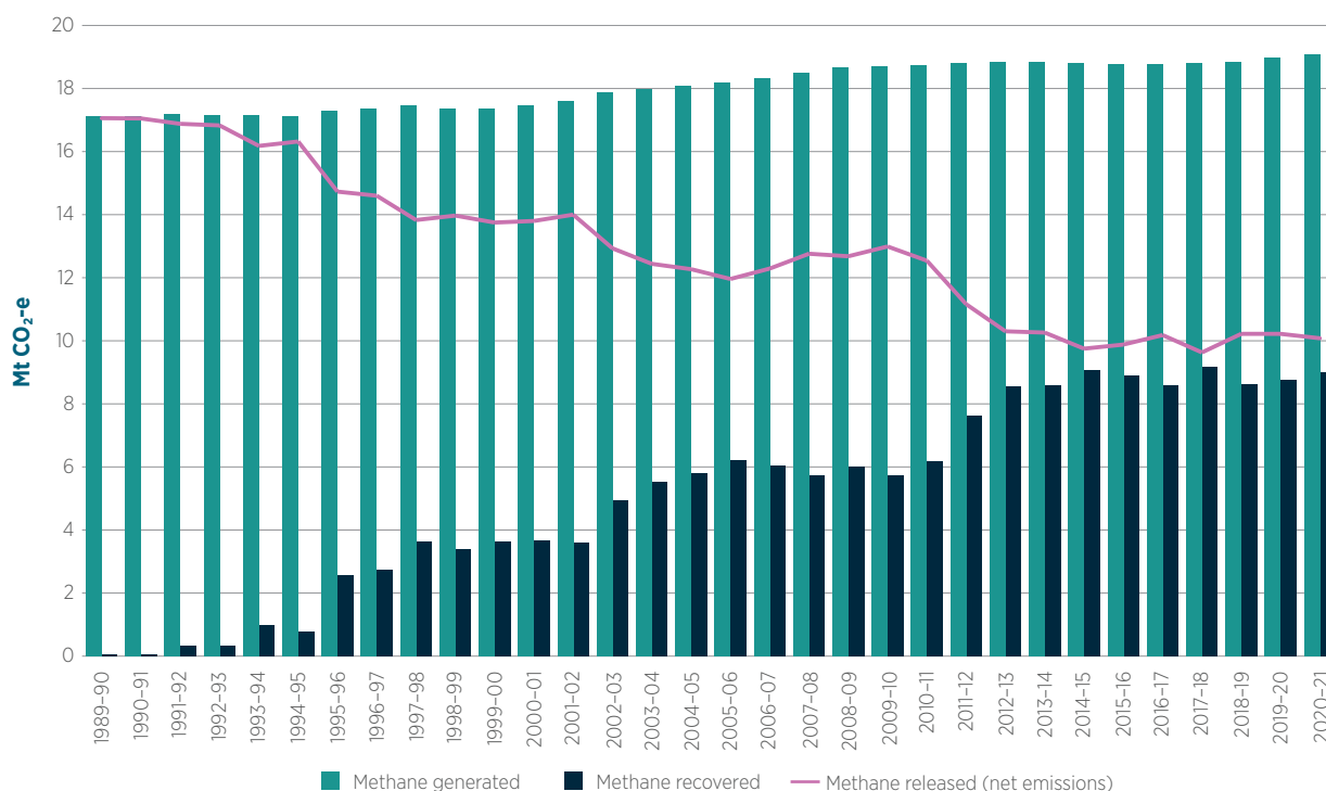
Figure 7.4 Trends in methane generation, recovery, and emissions from solid waste disposal, 1989–90 to 2020–21
