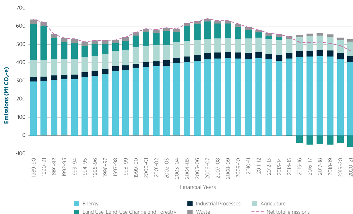
Figure ES.02 Greenhouse gas emissions by sector, Australia, 1989-90 to 2020-21 (Mt CO 2 -e)
