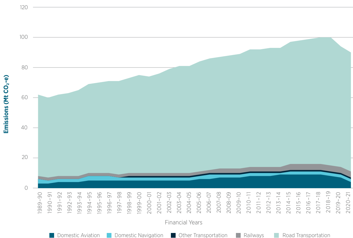
Figure 3.16 Transport emissions by subsector, 1989–90 to 2020–21
