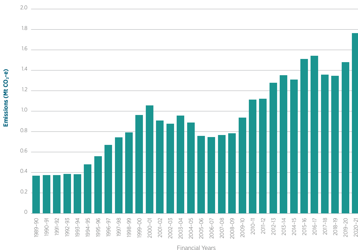
Figure 5.15 Emissions from urea application, Australia, Mt CO 2 -e
