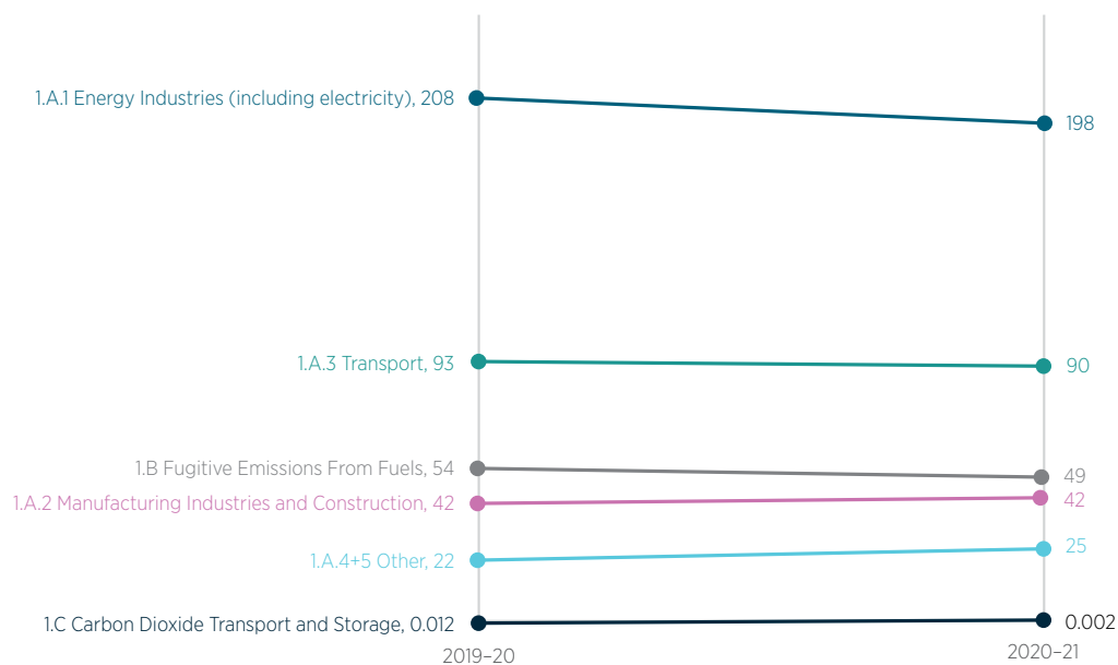
Figure 3.3 Slope chart comparing emissions by energy sub-sector in 2019-20 and 2020-21, Australia, Mt CO 2 -e
