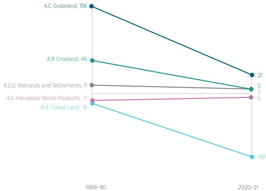
Figure 6.1.2 Slope chart comparing emissions by LULUCF sub-sector in 1989-90 and 2020-21, Australia, Mt CO 2 -e
