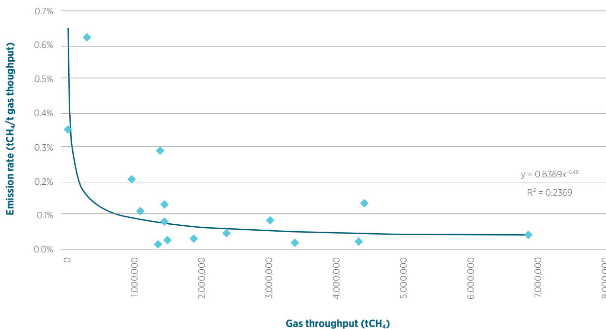
Figure 3.40 Gas processing plants with reported high emission rates are likely to have negligible gas throughputs
