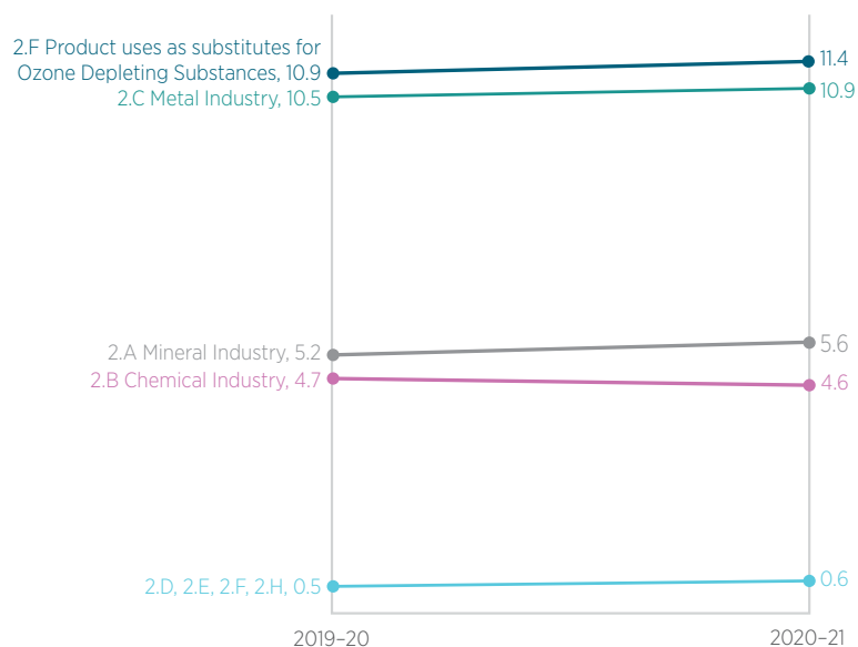
Figure 4.4 Slope chart comparing emissions by IPPU sub-sector in 2019–20 and 2020–21, Australia, Mt CO 2 -e
