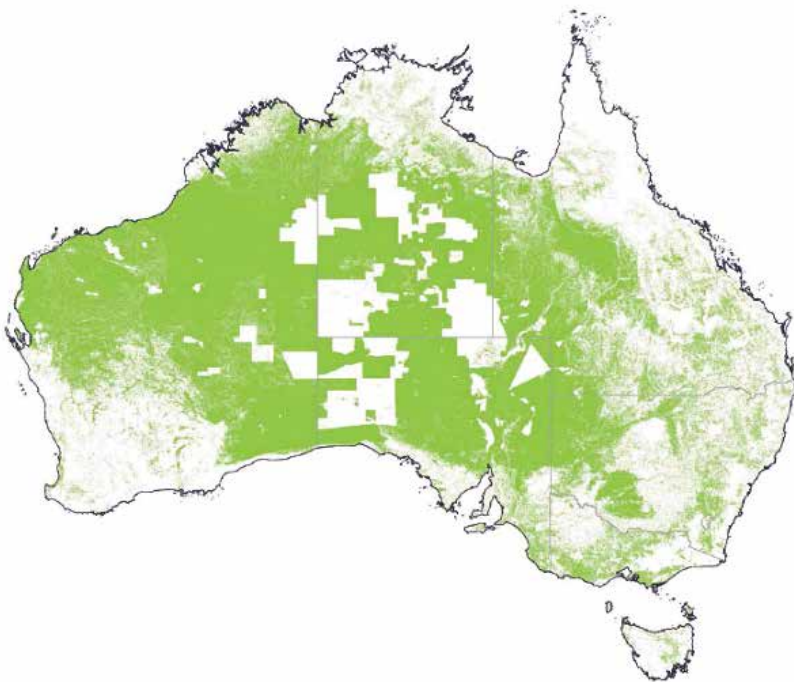
Figure 6.2.6 Grassland remaining grassland distribution in Australia
