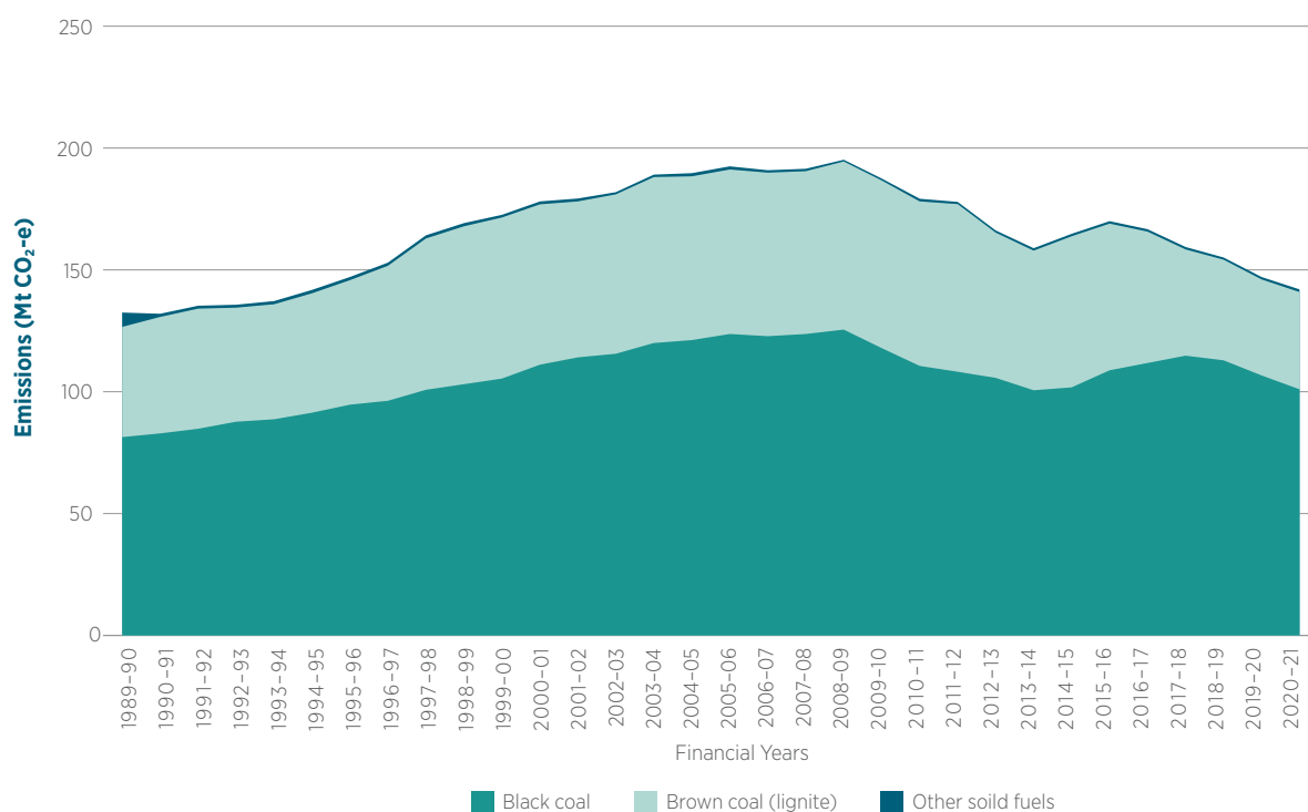
Figure 3.6 Emissions from solid fuel combustion, 1989–90 to 2020–21
