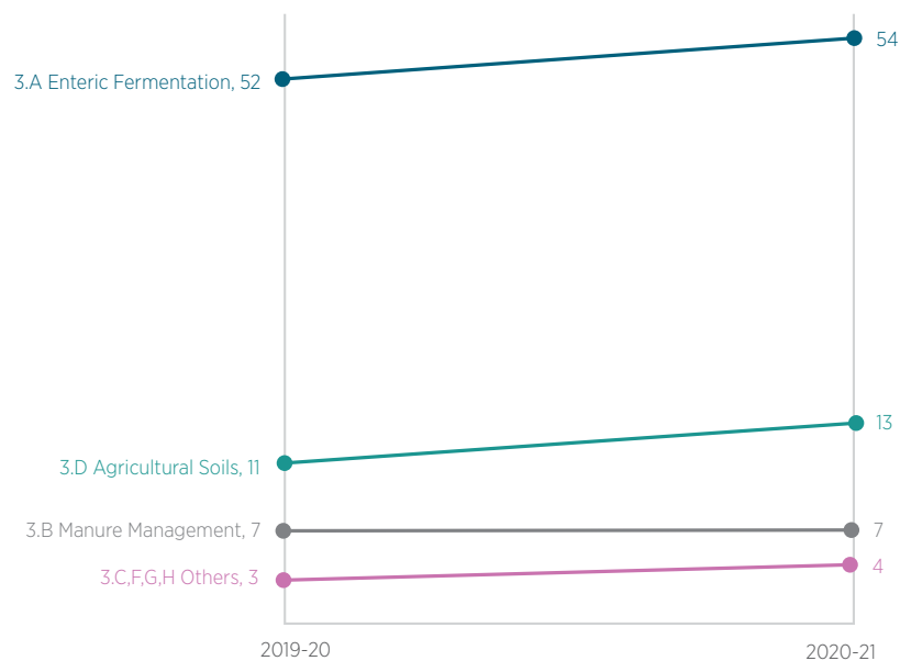
Figure 5.2 Slope chart comparing emissions by agriculture sub-sector in 2019-20 and 2020-21, Australia, Mt CO 2 -e
