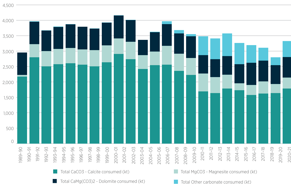
Figure 4.7 Carbonate consumption by type, Australia, 1989-90 to 2020-21, kt
