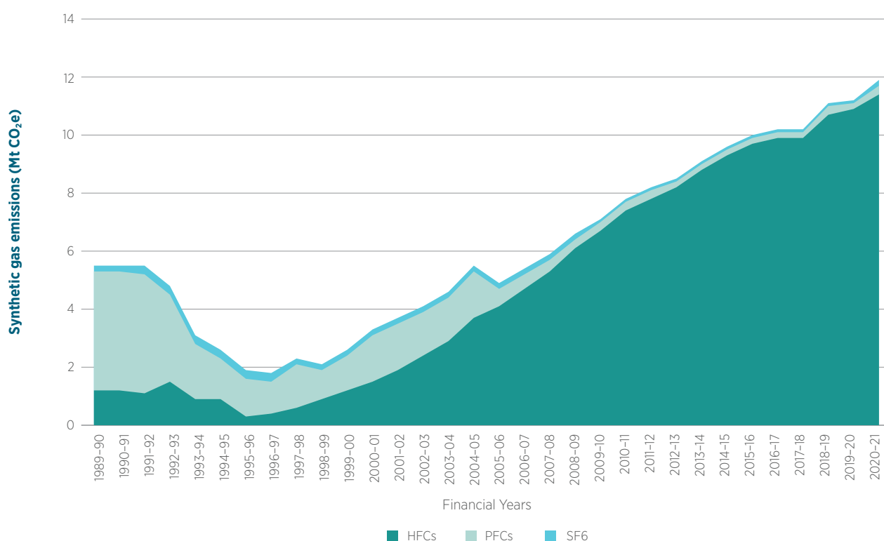
Figure 2.7 Synthetic gas emissions by year, Australia, Mt CO 2 -e
