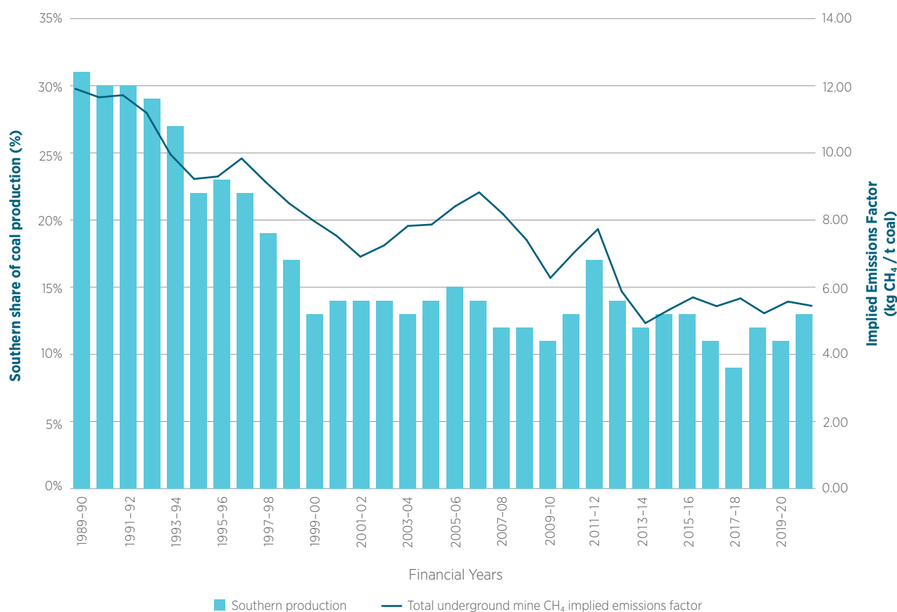
Figure 3.32 Decline of the overall underground coal mine methane implied emission factor compared with the fall in production from the high gas content Southern Coalfield
