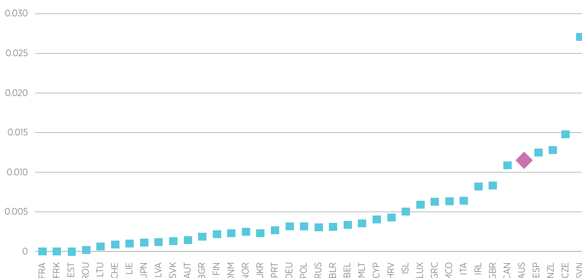
Figure 4.20 N 2 O use implied per capita emission factors or Annex I countries (2022 submission) and Australia (2023 submission), kt of CO 2 -e per thousand persons
