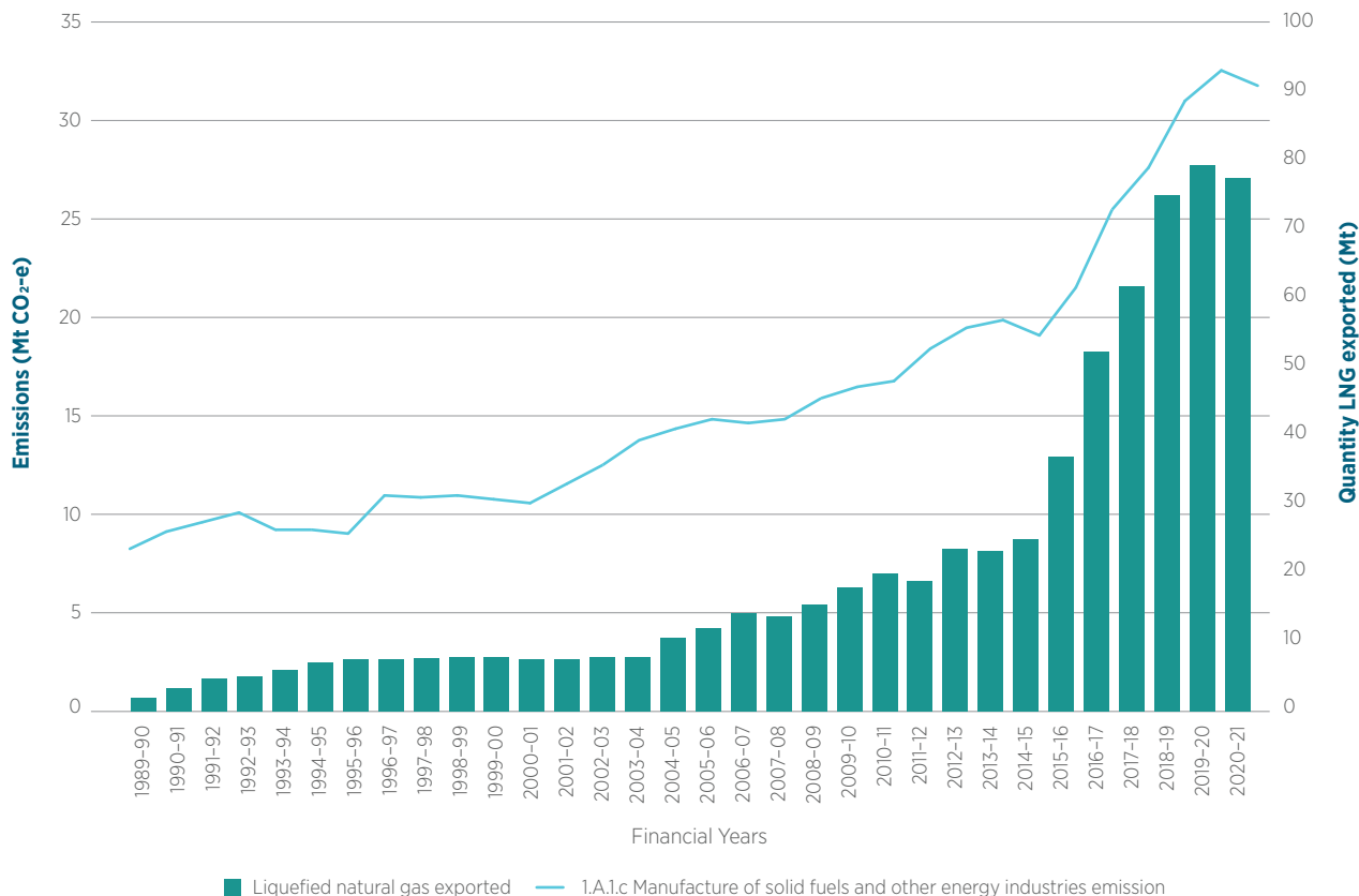
Figure 3.13 Emissions from the manufacture of solid fuels and other energy industries, and liquefied natural gas exports
