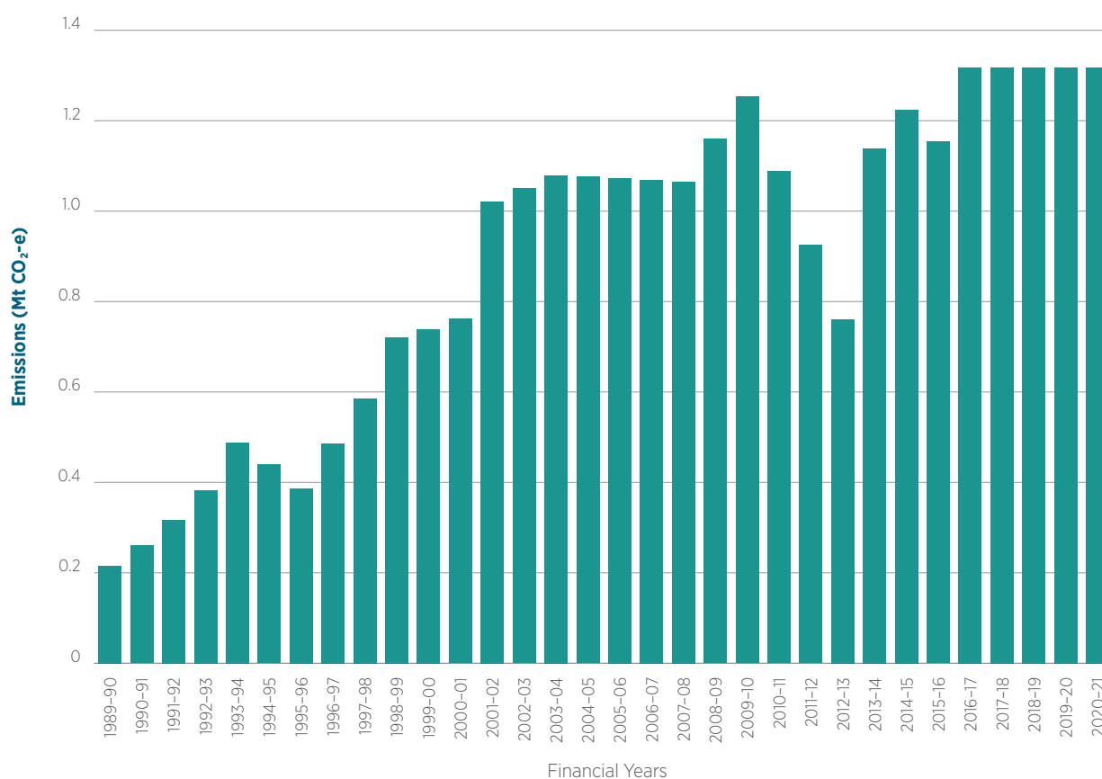
Figure 5.14 Emissions from liming, Australia, Mt CO 2 -e
