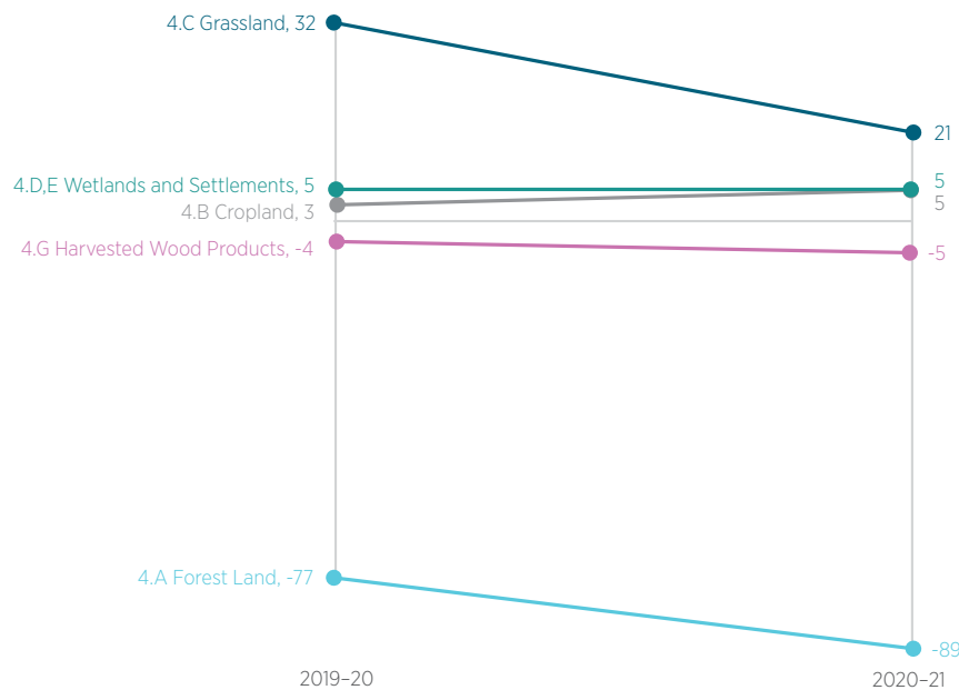
Figure 6.1.1 Slope chart comparing emissions by LULUCF sub-sector in 2019–20 and 2020–21, Australia, Mt CO 2 -e
