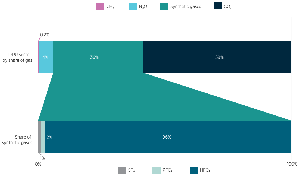
Figure 4.2 Gases as a share of total emissions within the Industrial Process and Product Use sector, CO 2 -e basis, 2020–21
