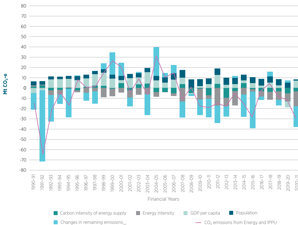
Figure 2.13 Annual change in total emissions from underlying drivers, Australia, 1990–91 to 2020–21, Mt CO 2 -e
