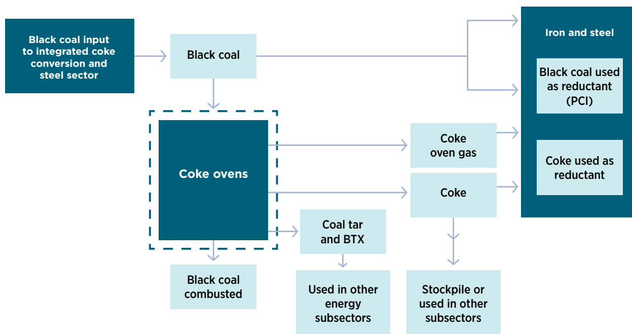
Figure 3.15 Coke Oven and Iron and Steel energy flow chart
