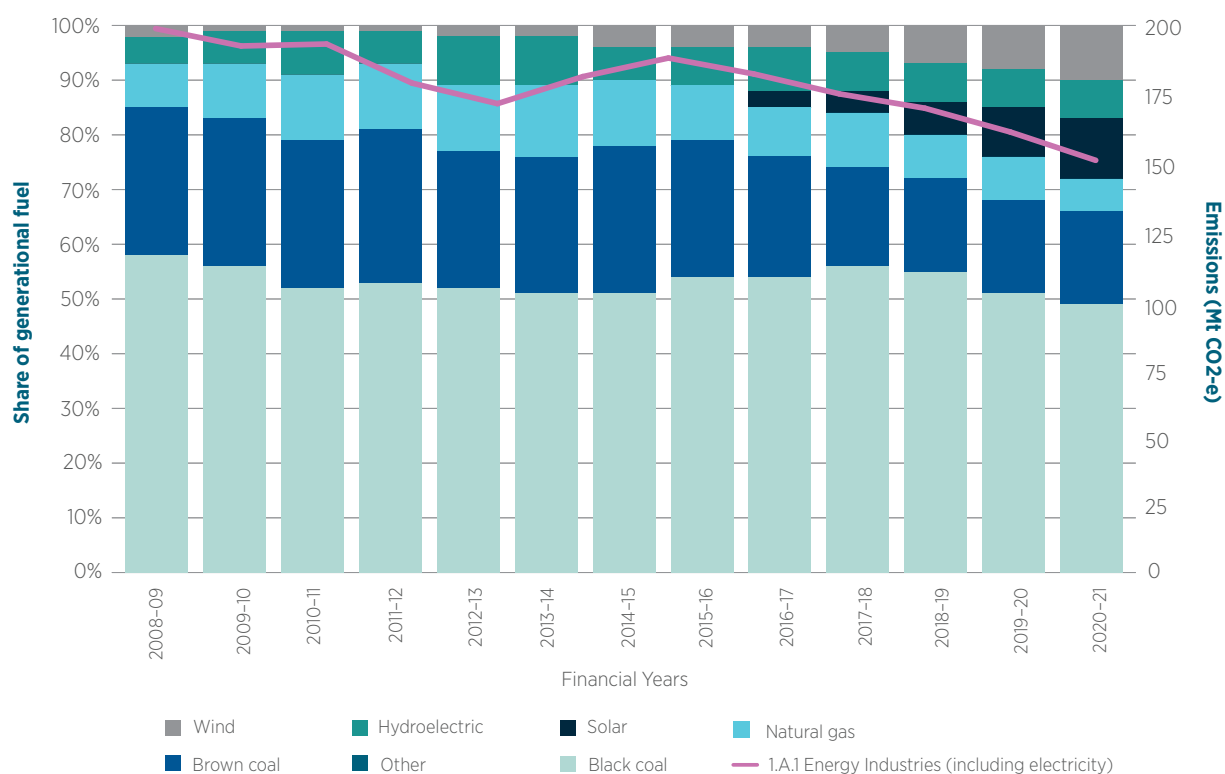
Figure 3.12 Emissions from electricity generation and shares of generation fuel since 2008–09
